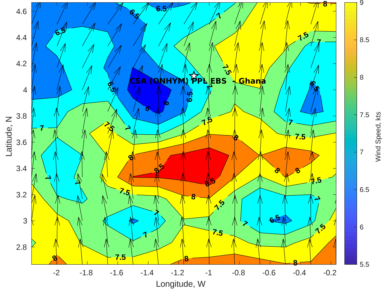
GFS Winds (kts) for CSA (ONHYM) PPL EBS - Ghana at 23-Dec-2025 09:00:00
