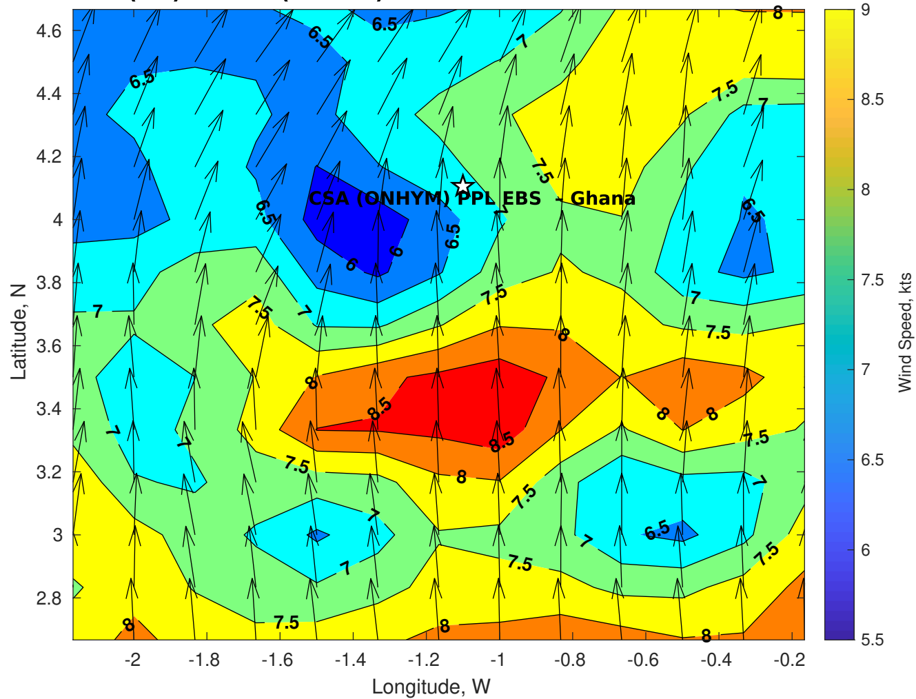
GFS Winds (kts) for CSA (ONHYM) PPL EBS - Ghana at 23-Dec-2025 09:00:00
