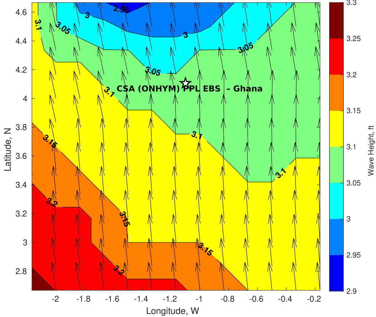
GFS Wave Height (ft) for CSA (ONHYM) PPL EBS - Ghana at 23-Dec-2025 09:00:00
