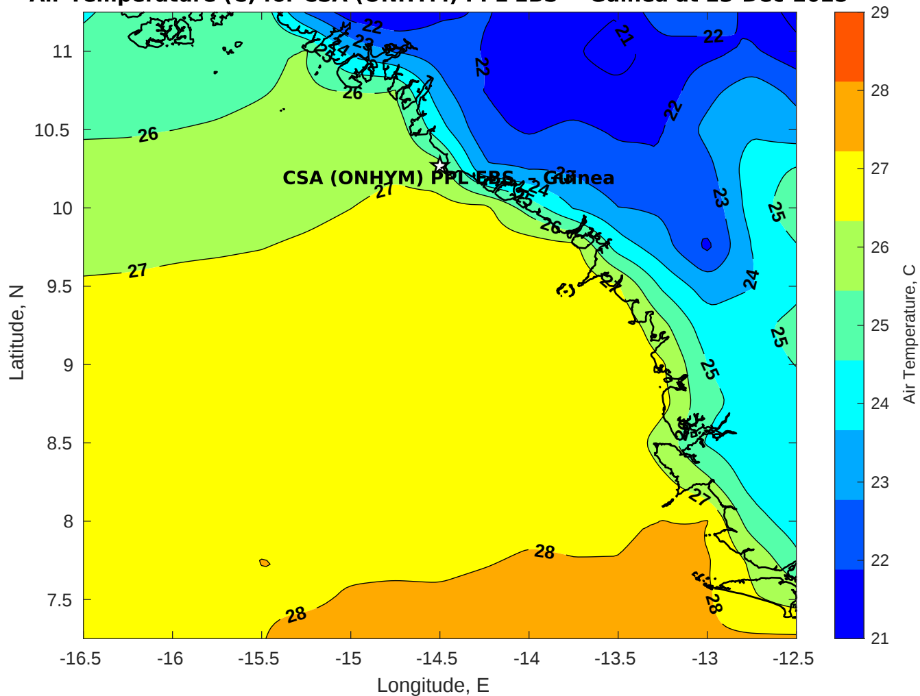
Air Temperature (C) for CSA (ONHYM) PPL EBS - Guinea at 23-Dec-2025
