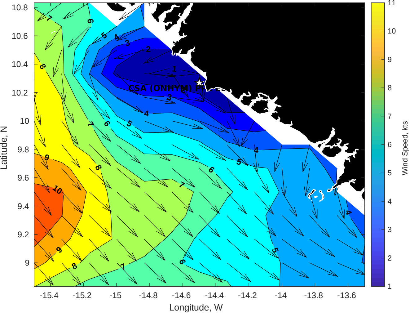
GFS Winds (kts) for CSA (ONHYM) PPL EBS - Guinea at 23-Dec-2025 09:00:00
