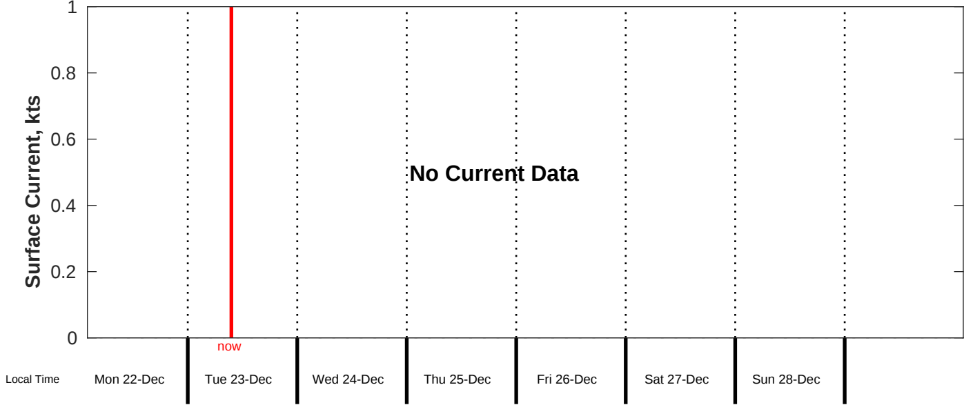
Surface Current Forecast for CSA (ONHYM) PPL EBS - Guinea from 22-Dec-2025 00:00:00 to 30-Dec-2025 00:00:00
