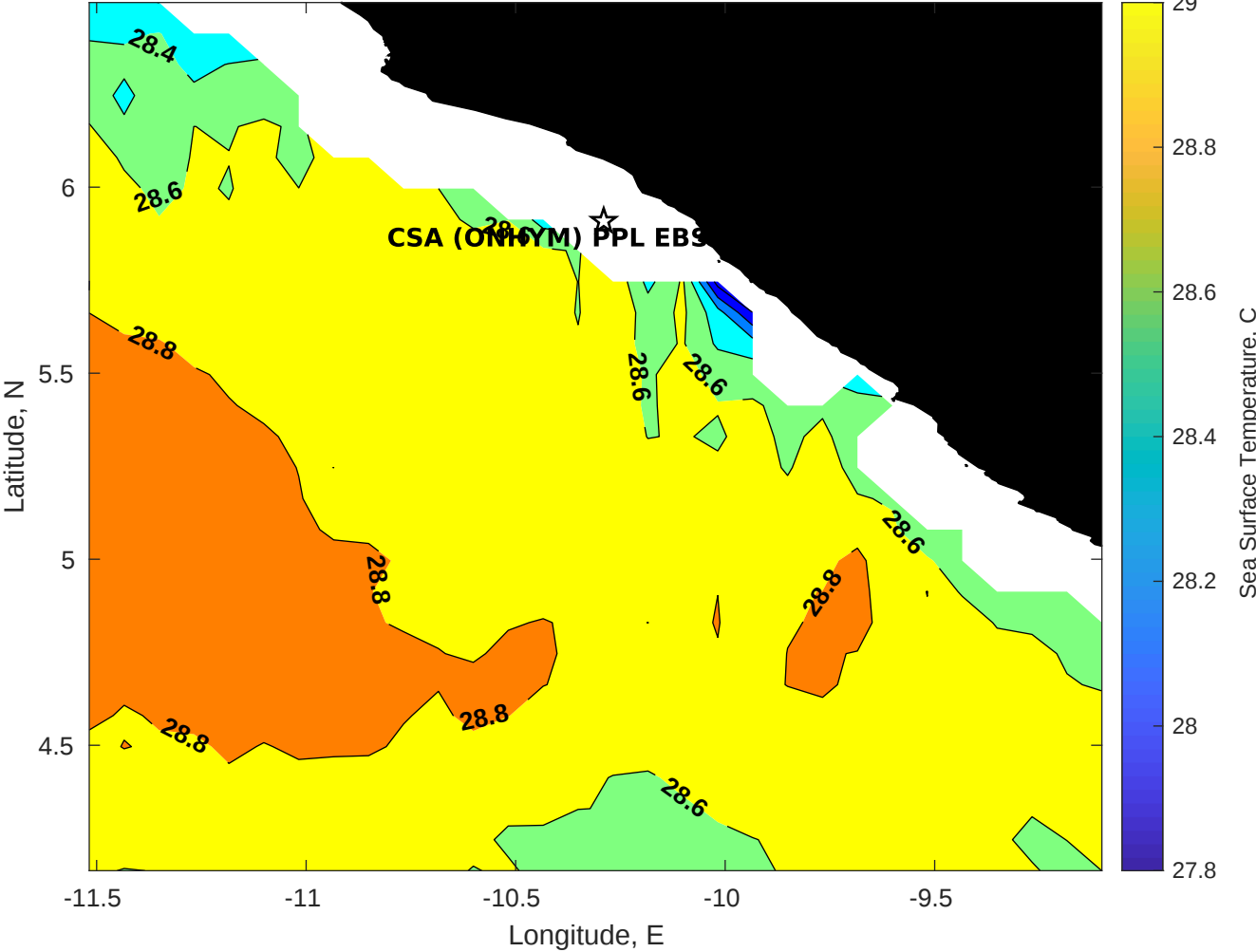
SST for CSA (ONHYM) PPL EBS - Liberia at 22-Dec-2025 00:00:00
