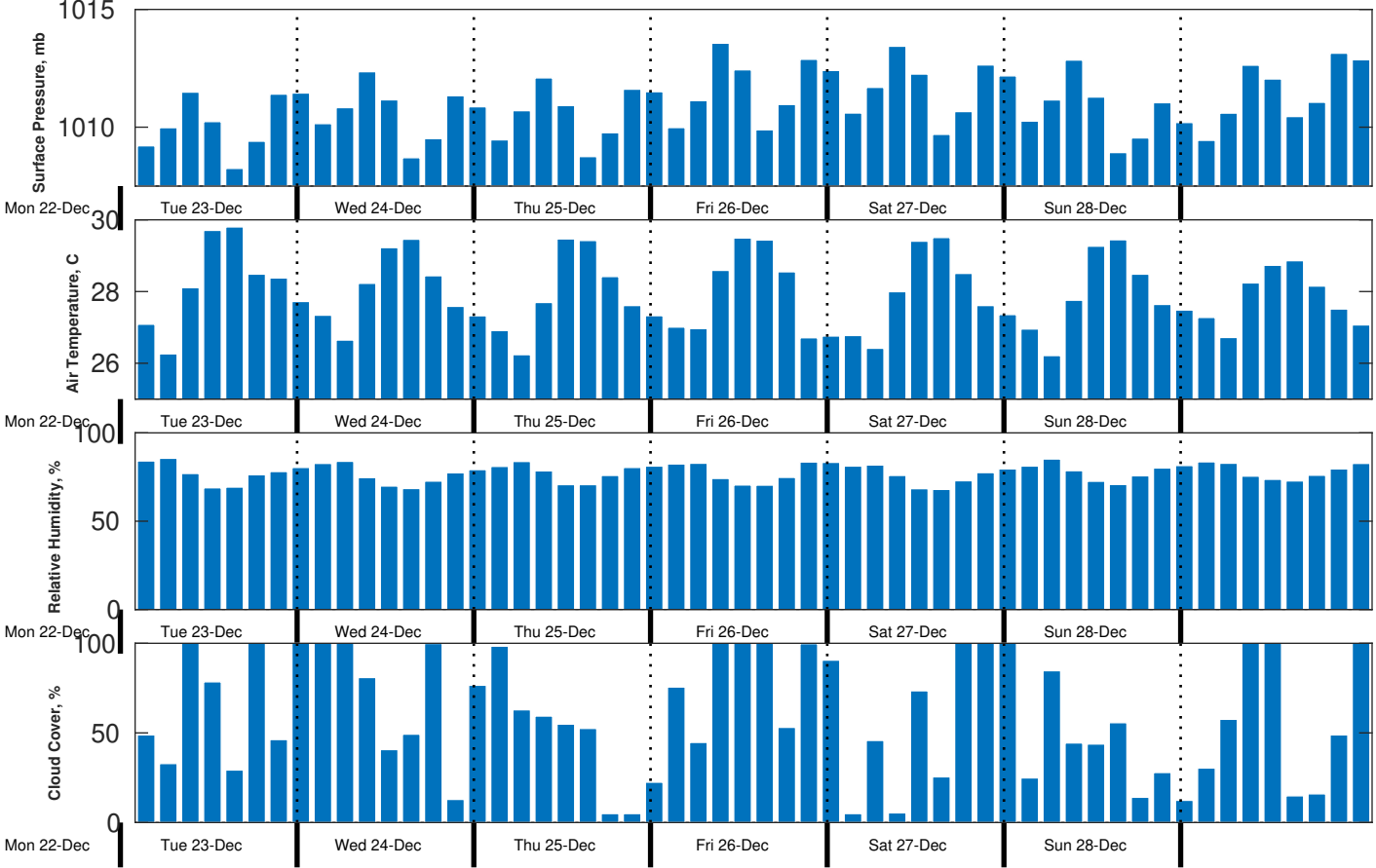
Met Forecast for CSA (ONHYM) PPL EBS - Liberia from 23-Dec-2025 00:00:00 to 30-Dec-2025 00:00:00
