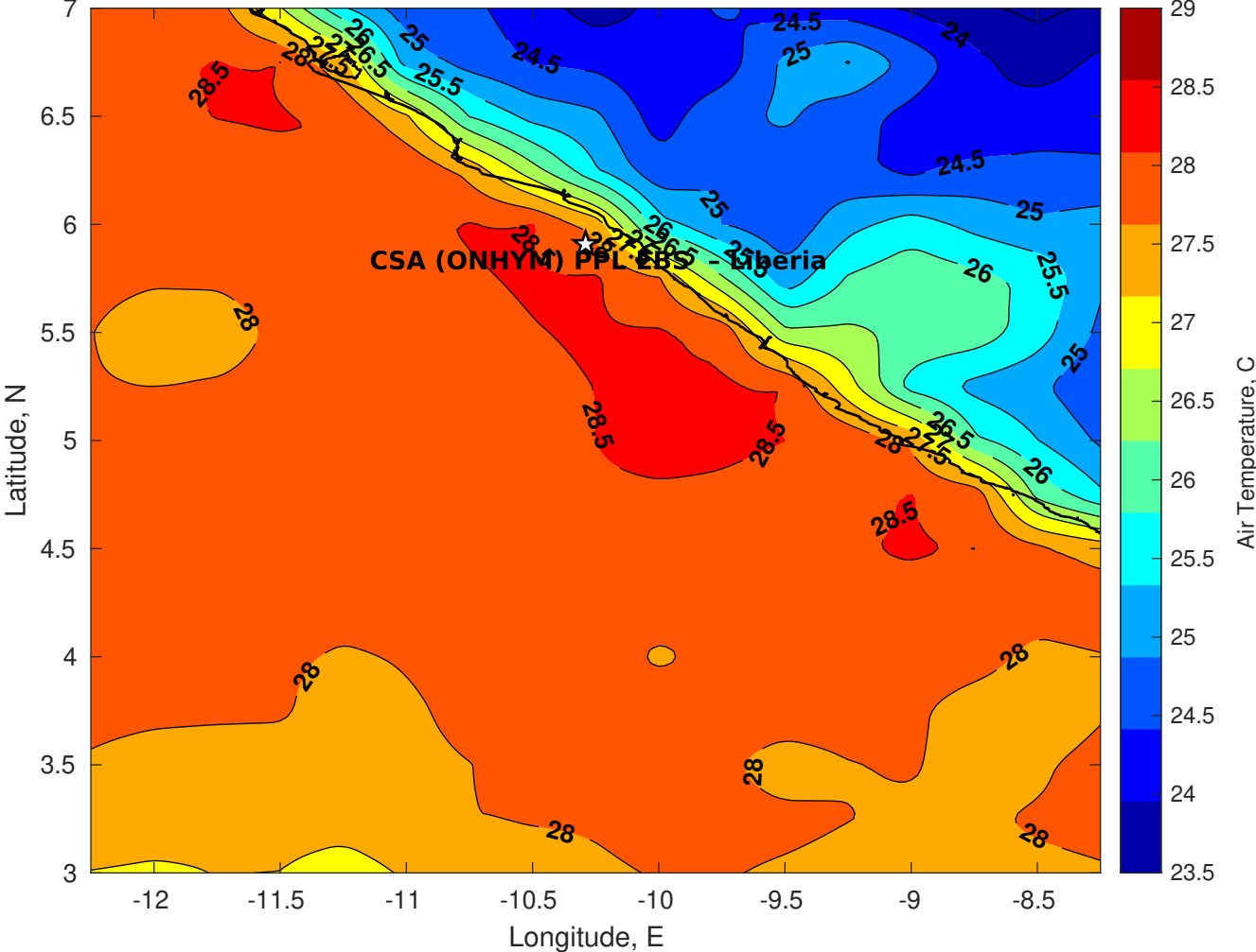
Air Temperature (C) for CSA (ONHYM) PPL EBS - Liberia at 23-Dec-2025
