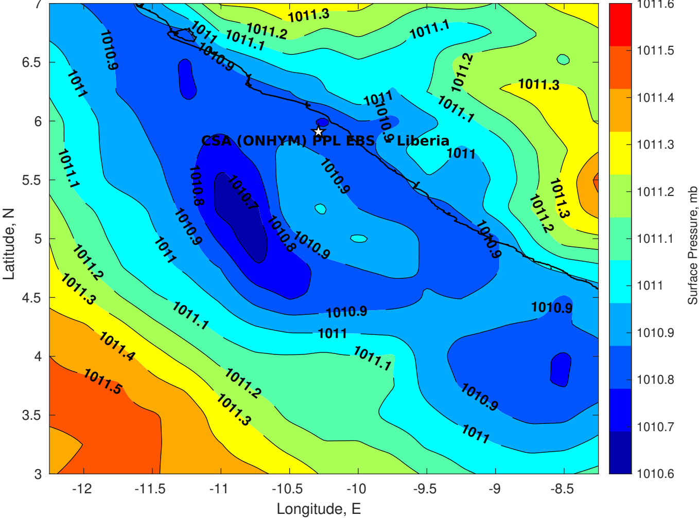
Surface Pressure (mb) for CSA (ONHYM) PPL EBS - Liberia at 23-Dec-2025 00:00:00
