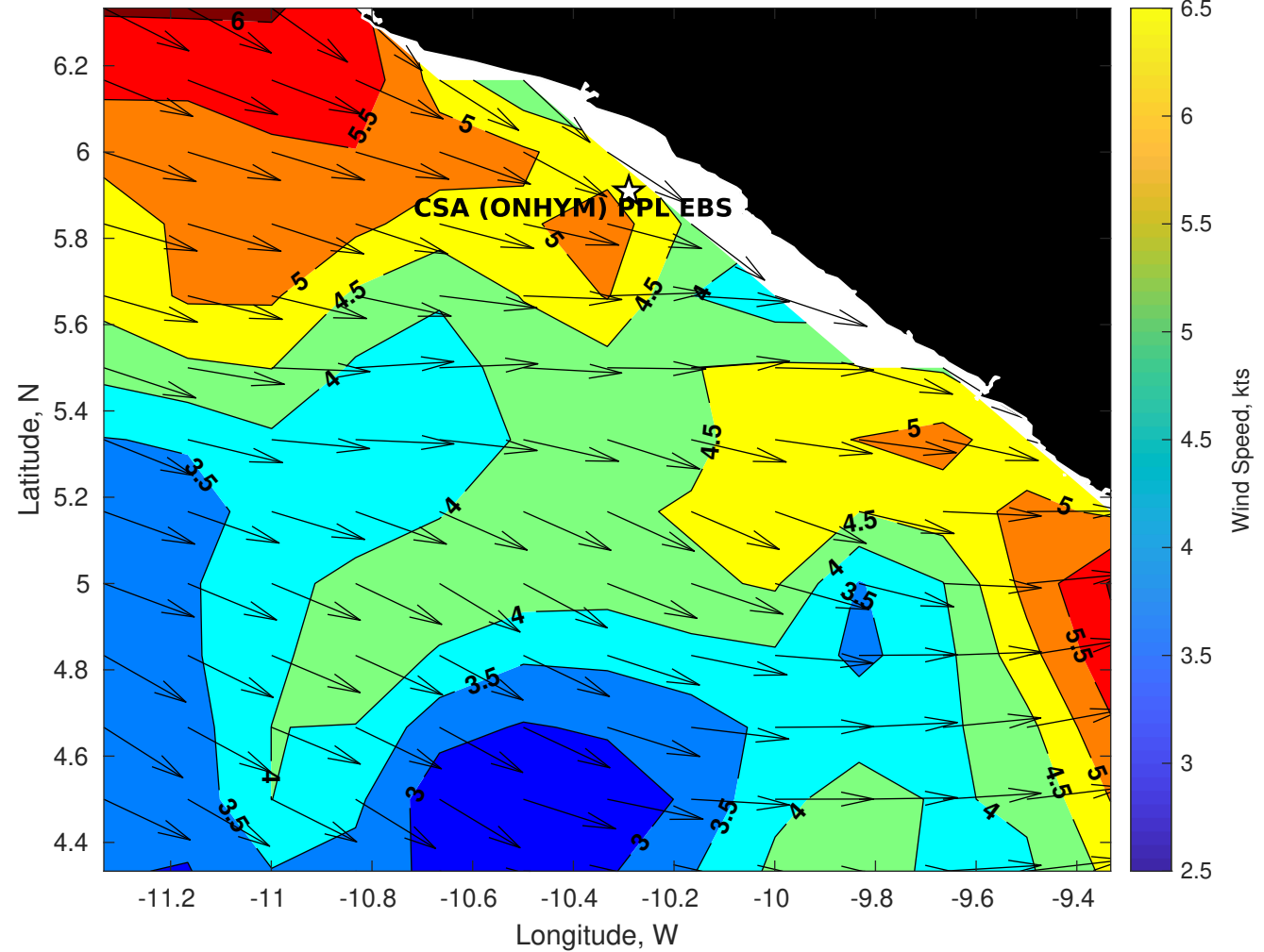
GFS Winds (kts) for CSA (ONHYM) PPL EBS - Liberia at 23-Dec-2025 09:00:00
