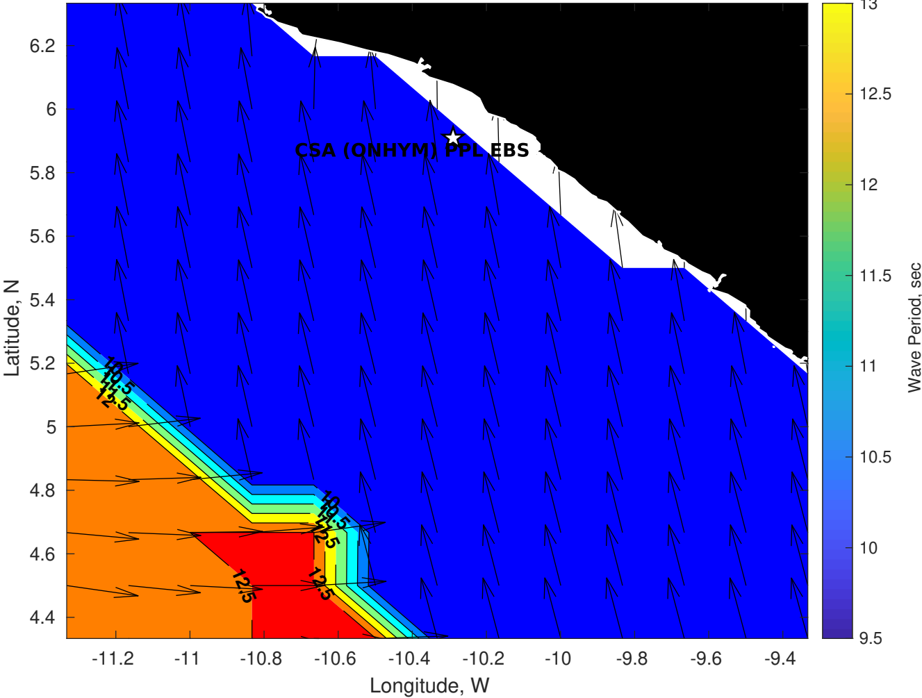
GFS Wave Period (sec) for CSA (ONHYM) PPL EBS - Liberia at 23-Dec-2025 09:00:00
