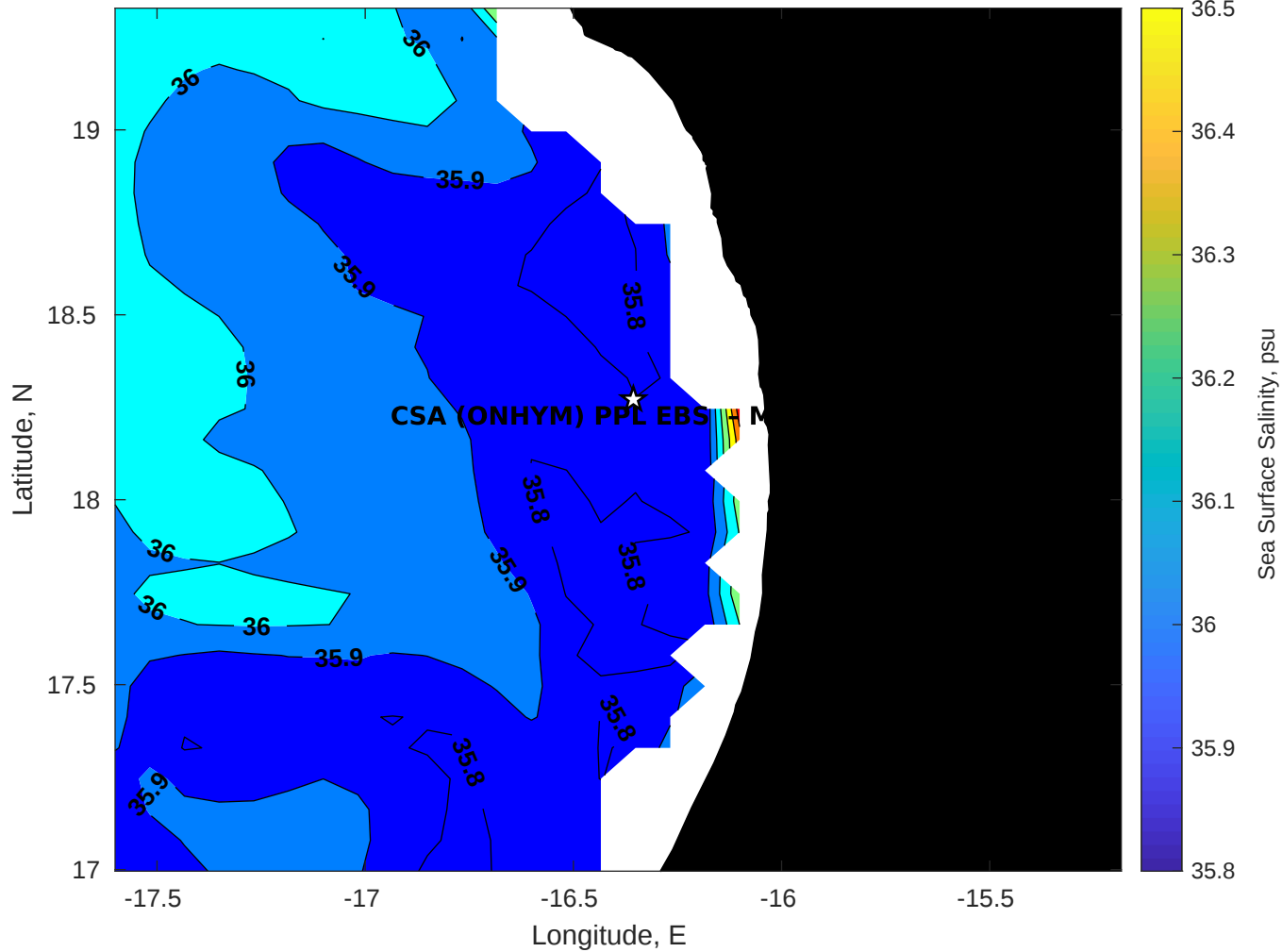
Surface Salinity for CSA (ONHYM) PPL EBS - Mauritania at 22-Dec-2025 00:00:00
