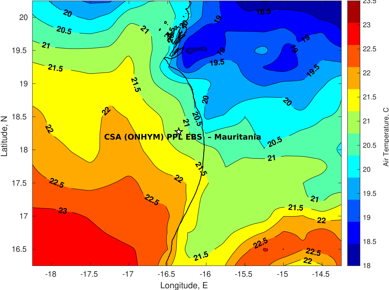
Air Temperature (C) for CSA (ONHYM) PPL EBS - Mauritania at 23-Dec-2025
