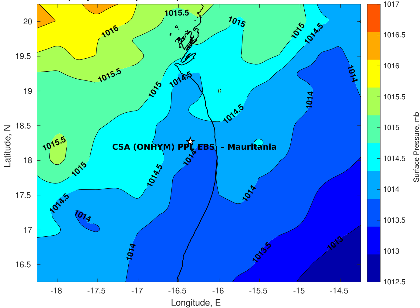
Surface Pressure (mb) for CSA (ONHYM) PPL EBS - Mauritania at 25-Dec-2025 00:00:00
