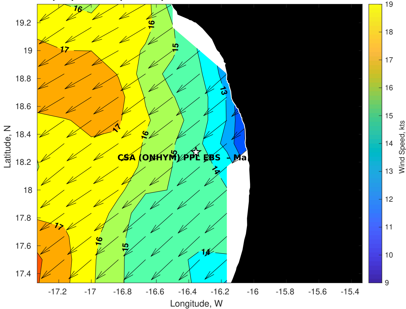
GFS Winds (kts) for CSA (ONHYM) PPL EBS - Mauritania at 23-Dec-2025 09:00:00
