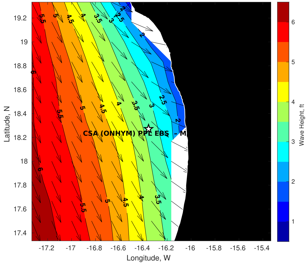
GFS Wave Height (ft) for CSA (ONHYM) PPL EBS - Mauritania at 23-Dec-2025 09:00:00
