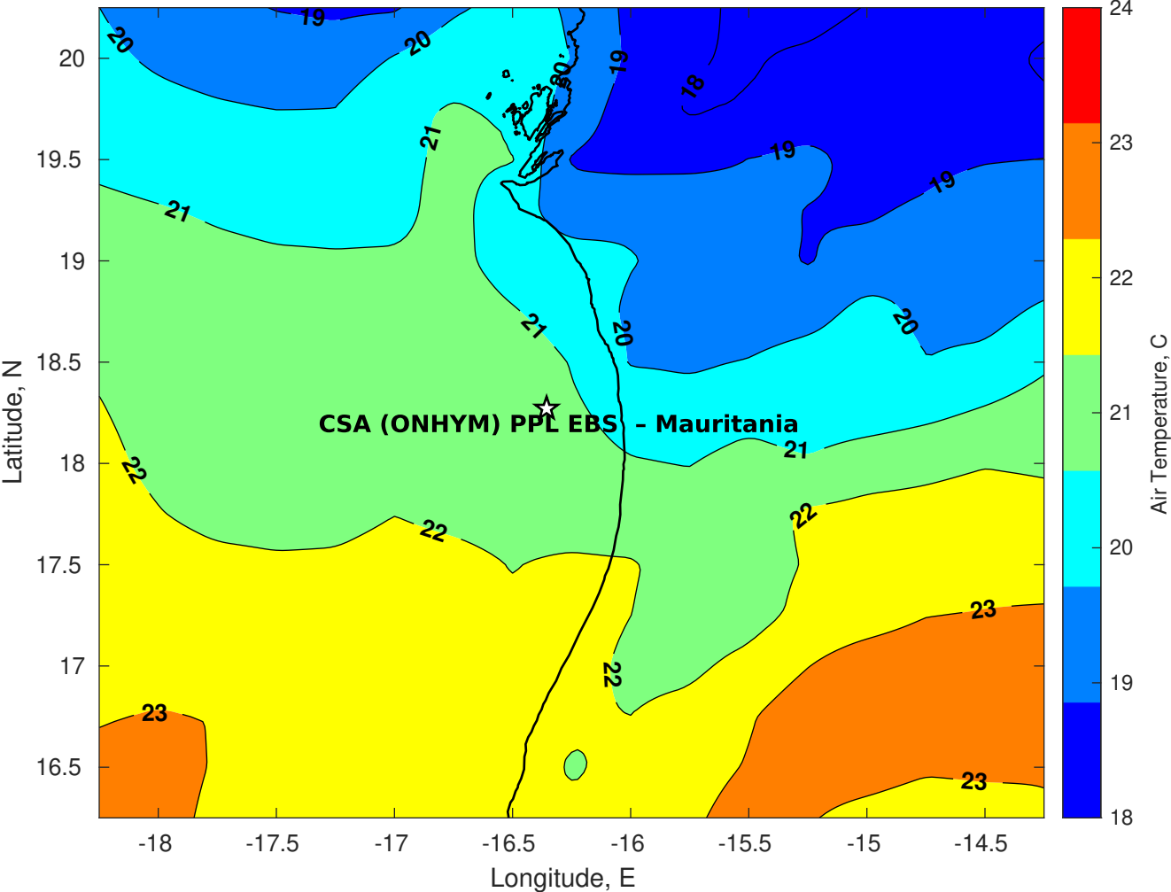
Air Temperature (C) for CSA (ONHYM) PPL EBS - Mauritania at 23-Dec-2025
