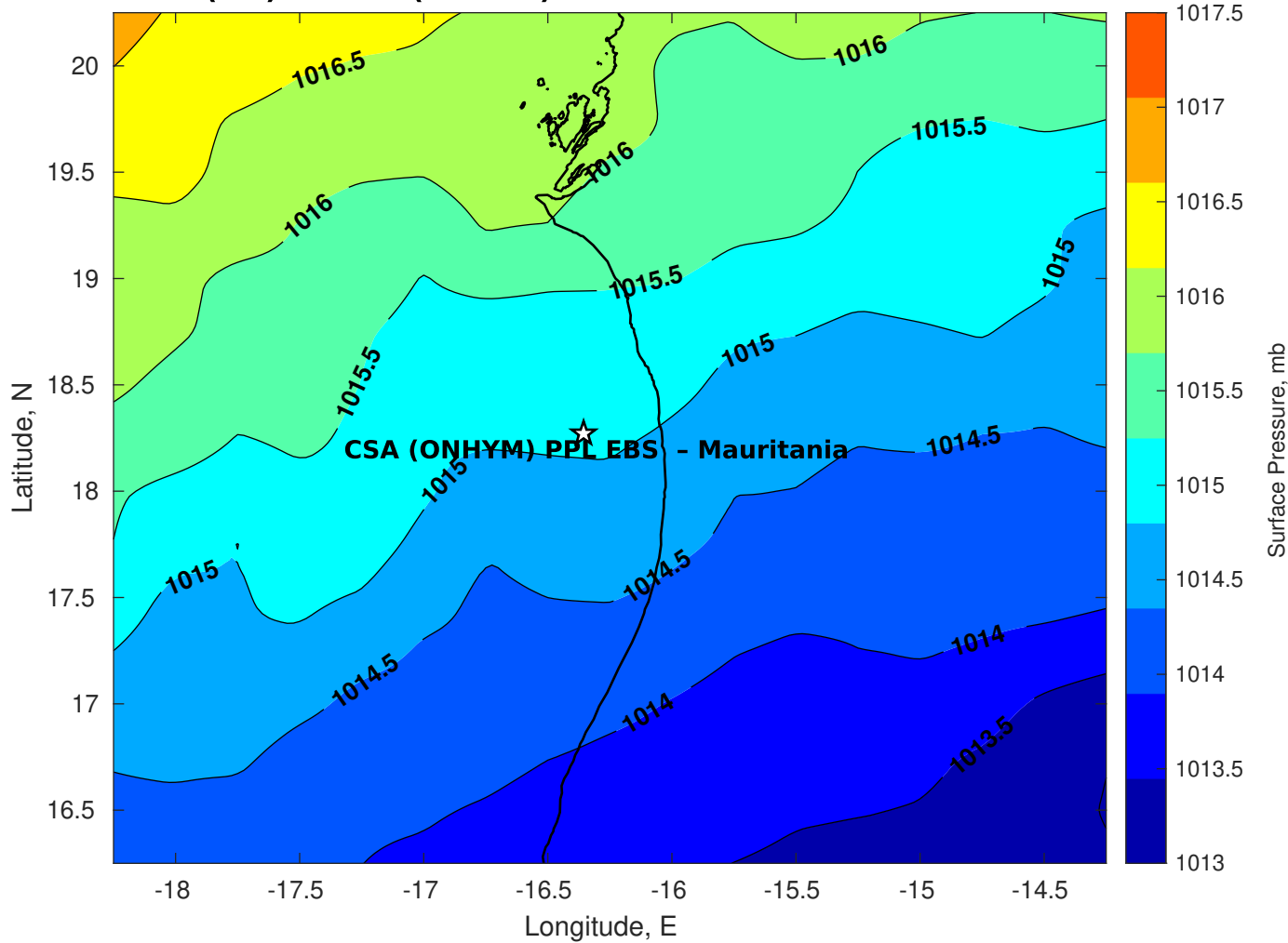
Surface Pressure (mb) for CSA (ONHYM) PPL EBS - Mauritania at 24-Dec-2025 00:00:00
