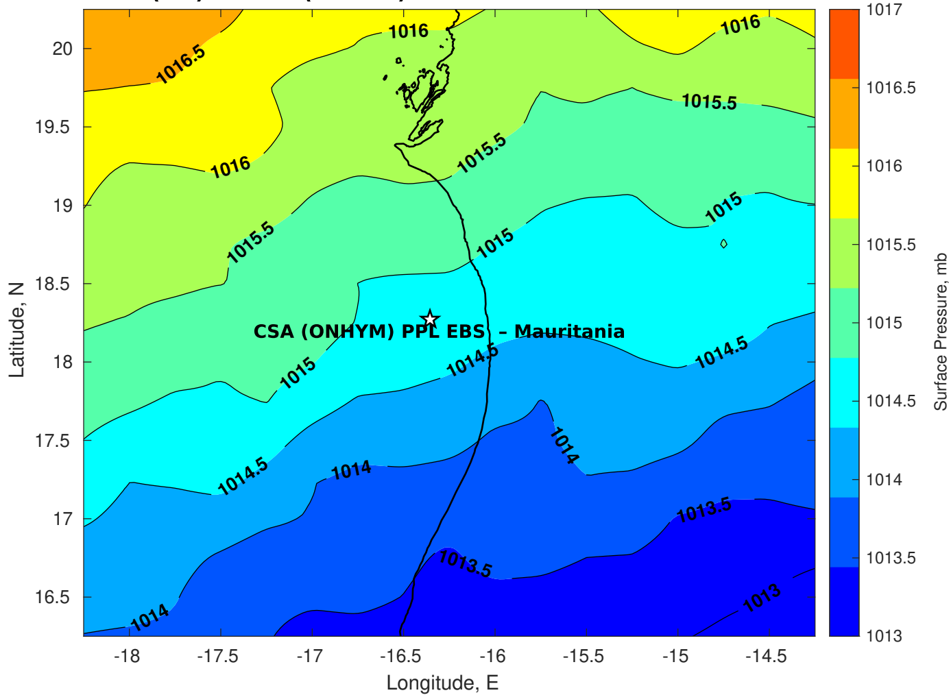
Surface Pressure (mb) for CSA (ONHYM) PPL EBS - Mauritania at 23-Dec-2025 00:00:00
