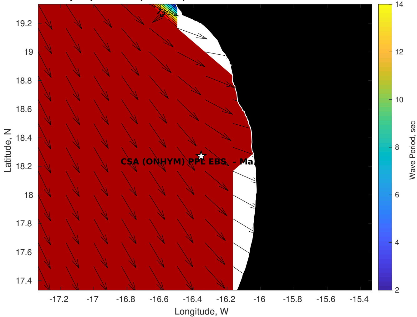
GFS Wave Period (sec) for CSA (ONHYM) PPL EBS - Mauritania at 23-Dec-2025 09:00:00
