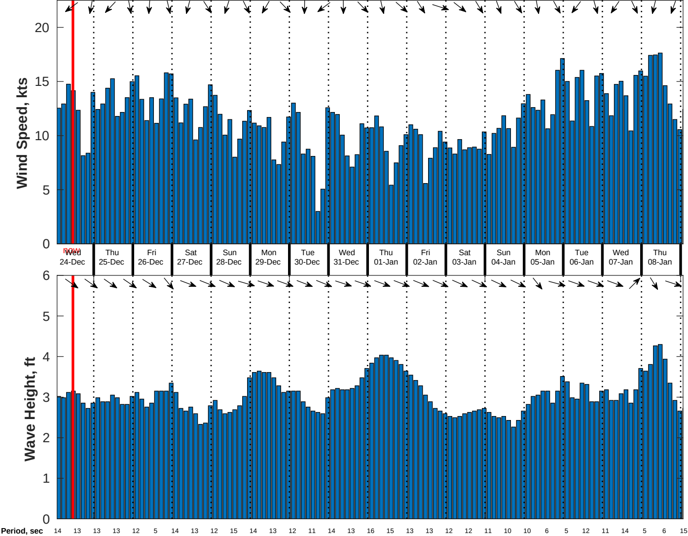
Wind & Wave Forecast for CSA (ONHYM) PPL EBS - Mauritania from 23-Dec-2025 01:00:00 to 08-Jan-2026 01:00:00
