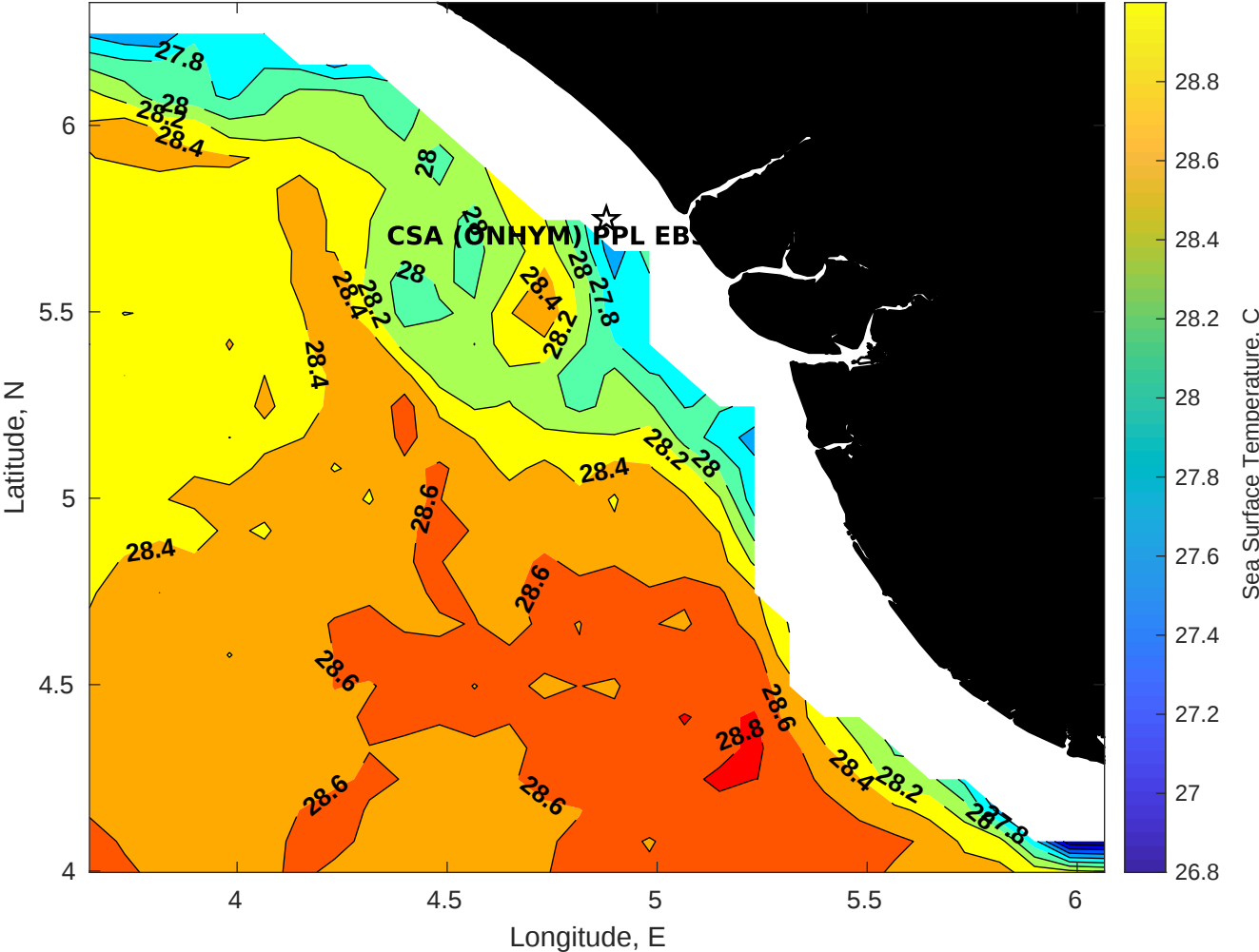
SST for CSA (ONHYM) PPL EBS - Nigeria at 22-Dec-2025 00:00:00
