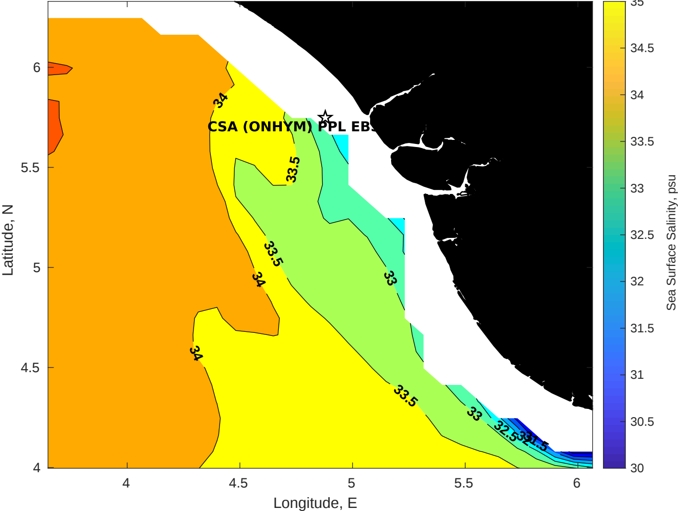
Surface Salinity for CSA (ONHYM) PPL EBS - Nigeria at 22-Dec-2025 00:00:00
