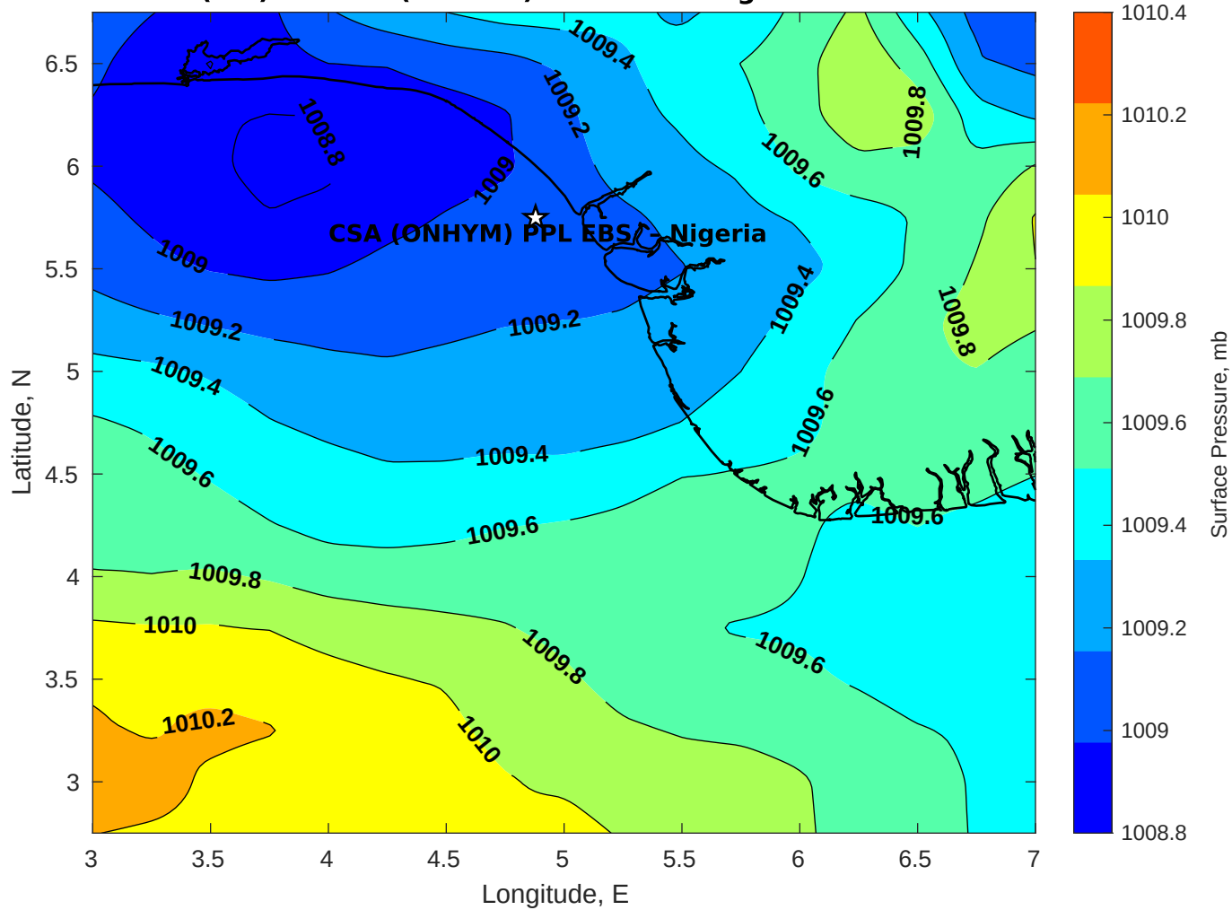
Surface Pressure (mb) for CSA (ONHYM) PPL EBS - Nigeria at 23-Dec-2025 00:00:00
