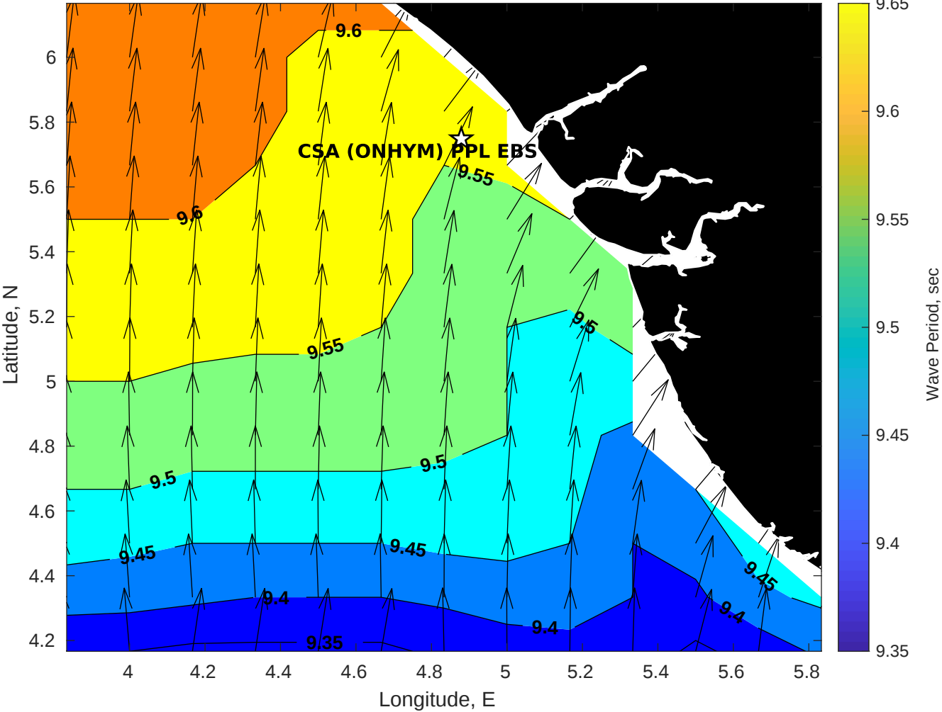
GFS Wave Period (sec) for CSA (ONHYM) PPL EBS - Nigeria at 23-Dec-2025 09:00:00
