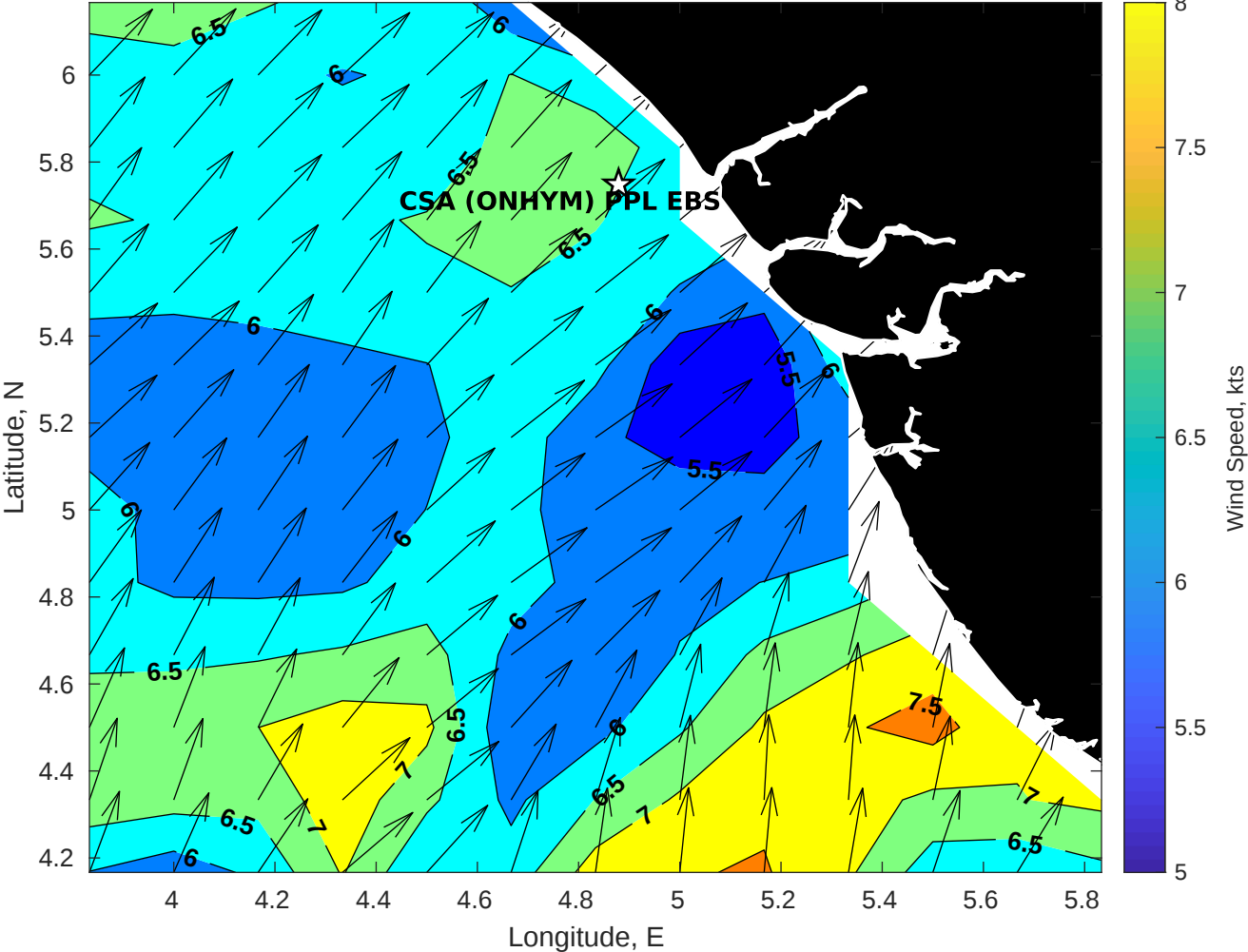
GFS Winds (kts) for CSA (ONHYM) PPL EBS - Nigeria at 23-Dec-2025 09:00:00
