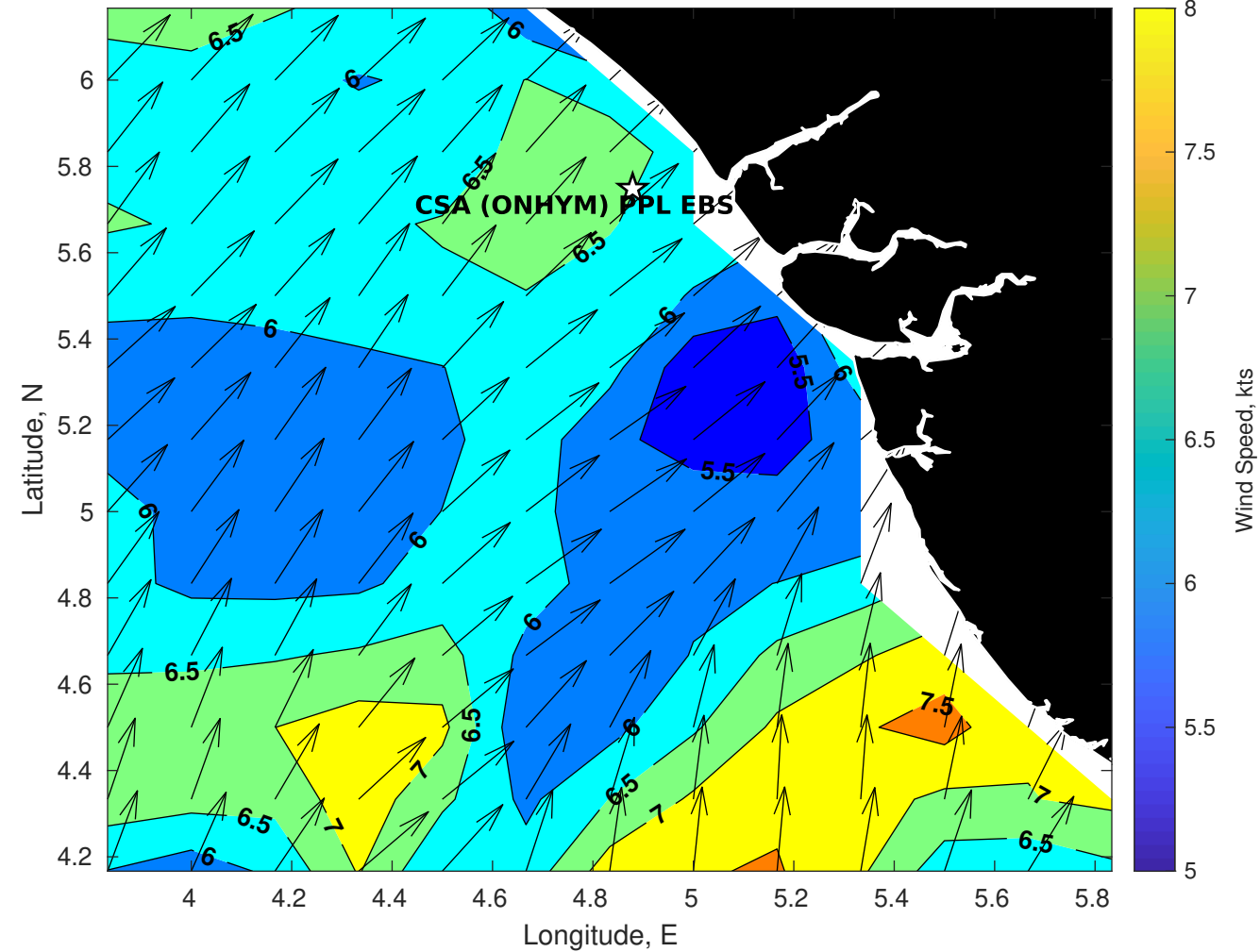
GFS Winds (kts) for CSA (ONHYM) PPL EBS - Nigeria at 23-Dec-2025 09:00:00
