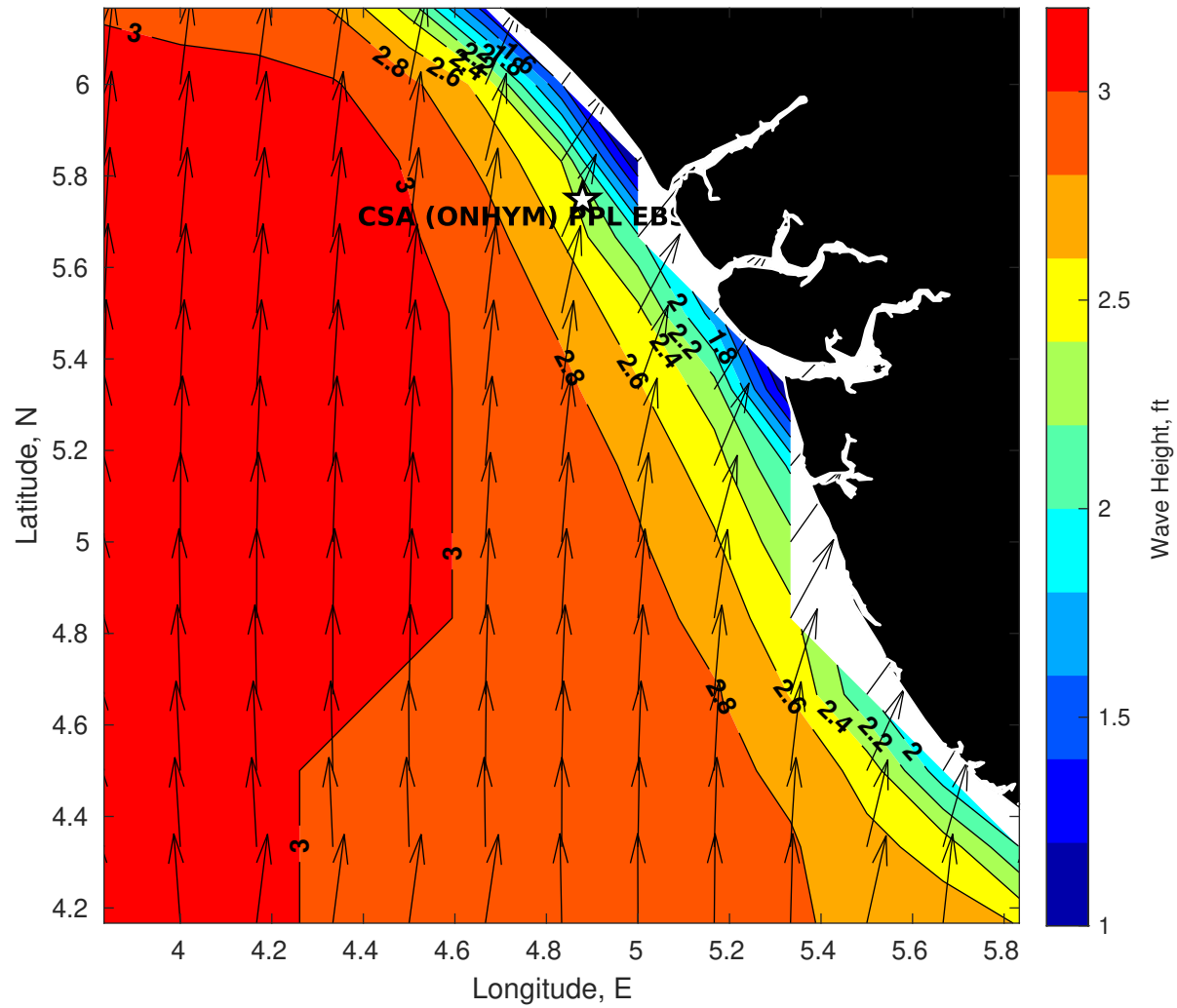
GFS Wave Height (ft) for CSA (ONHYM) PPL EBS - Nigeria at 23-Dec-2025 09:00:00
