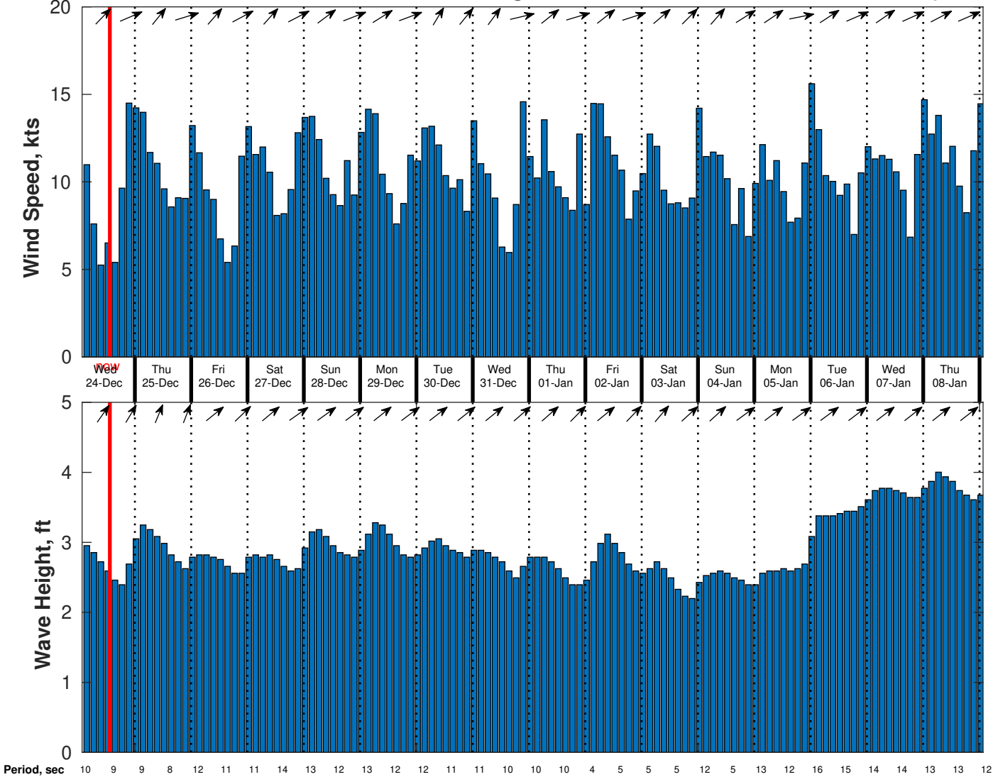
Wind & Wave Forecast for CSA (ONHYM) PPL EBS - Nigeria from 23-Dec-2025 02:00:00 to 08-Jan-2026 02:00:00
