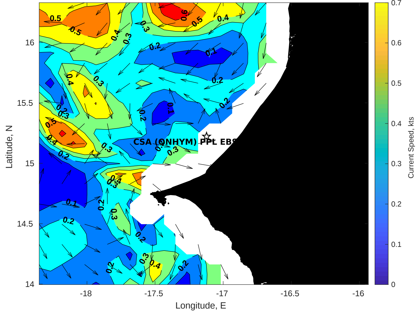
Surface Currents for CSA (ONHYM) PPL EBS - Senegal at 22-Dec-2025 00:00:00
