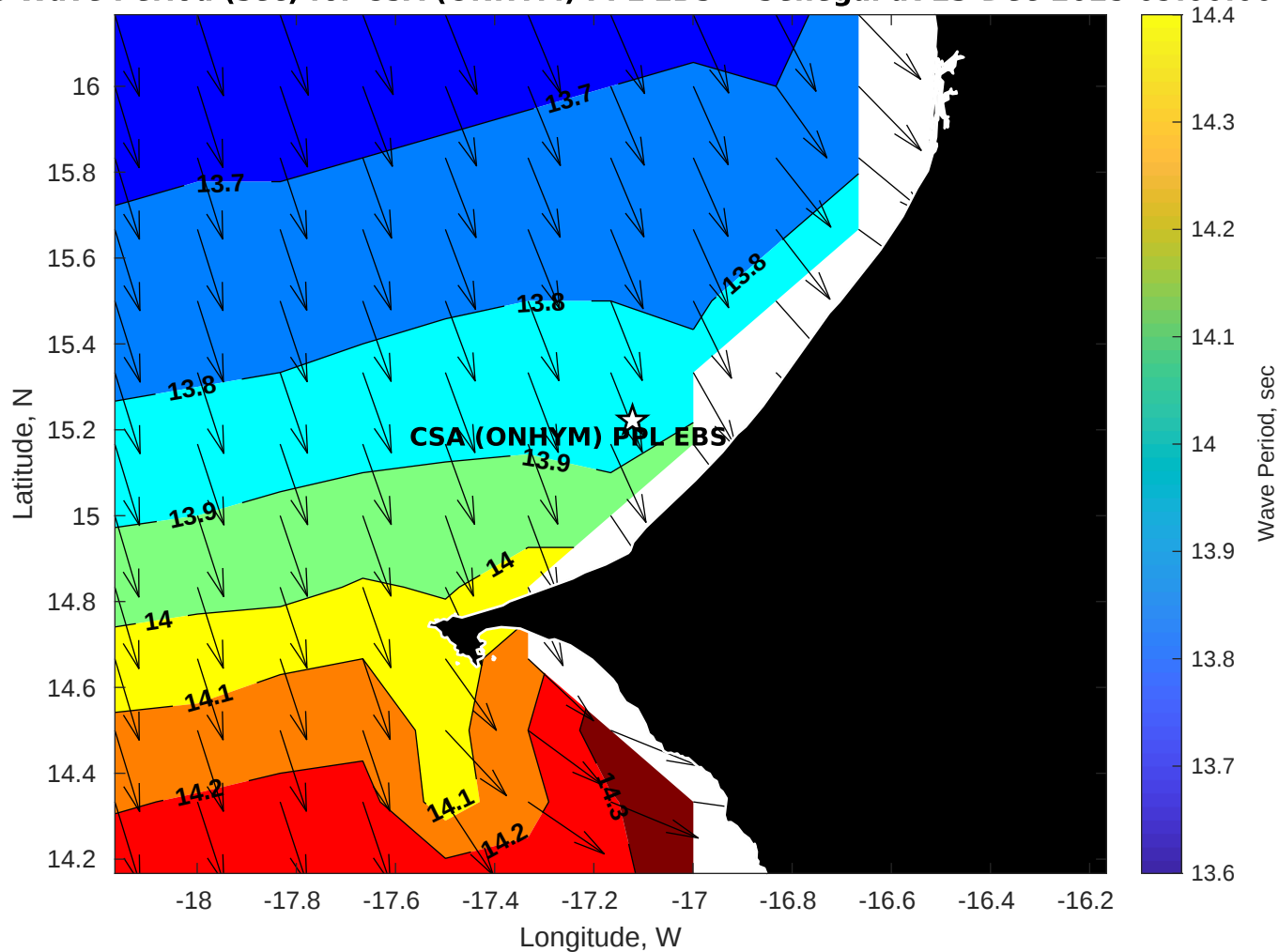
GFS Wave Period (sec) for CSA (ONHYM) PPL EBS - Senegal at 23-Dec-2025 09:00:00
