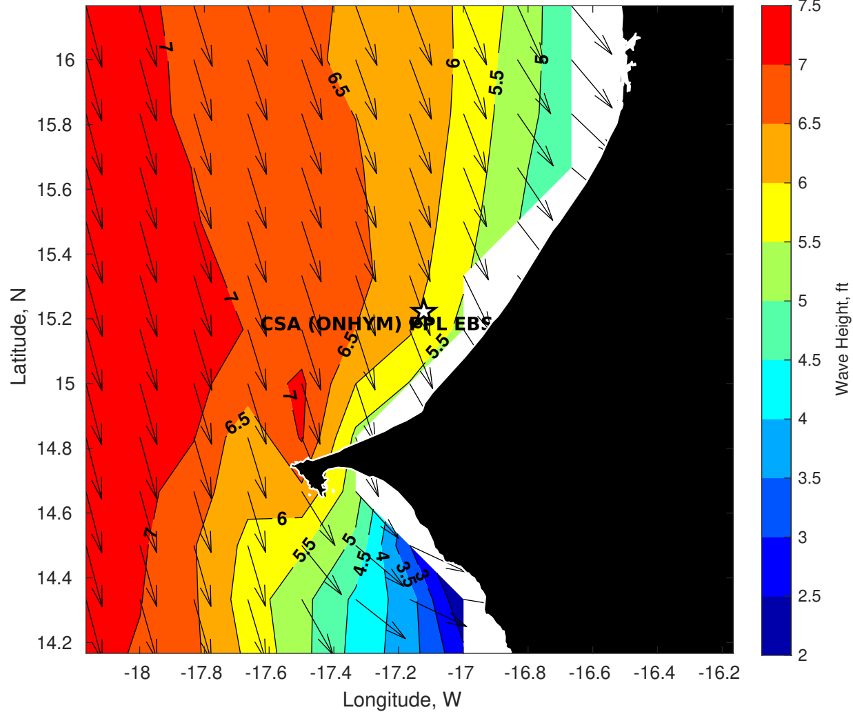
GFS Wave Height (ft) for CSA (ONHYM) PPL EBS - Senegal at 23-Dec-2025 09:00:00
