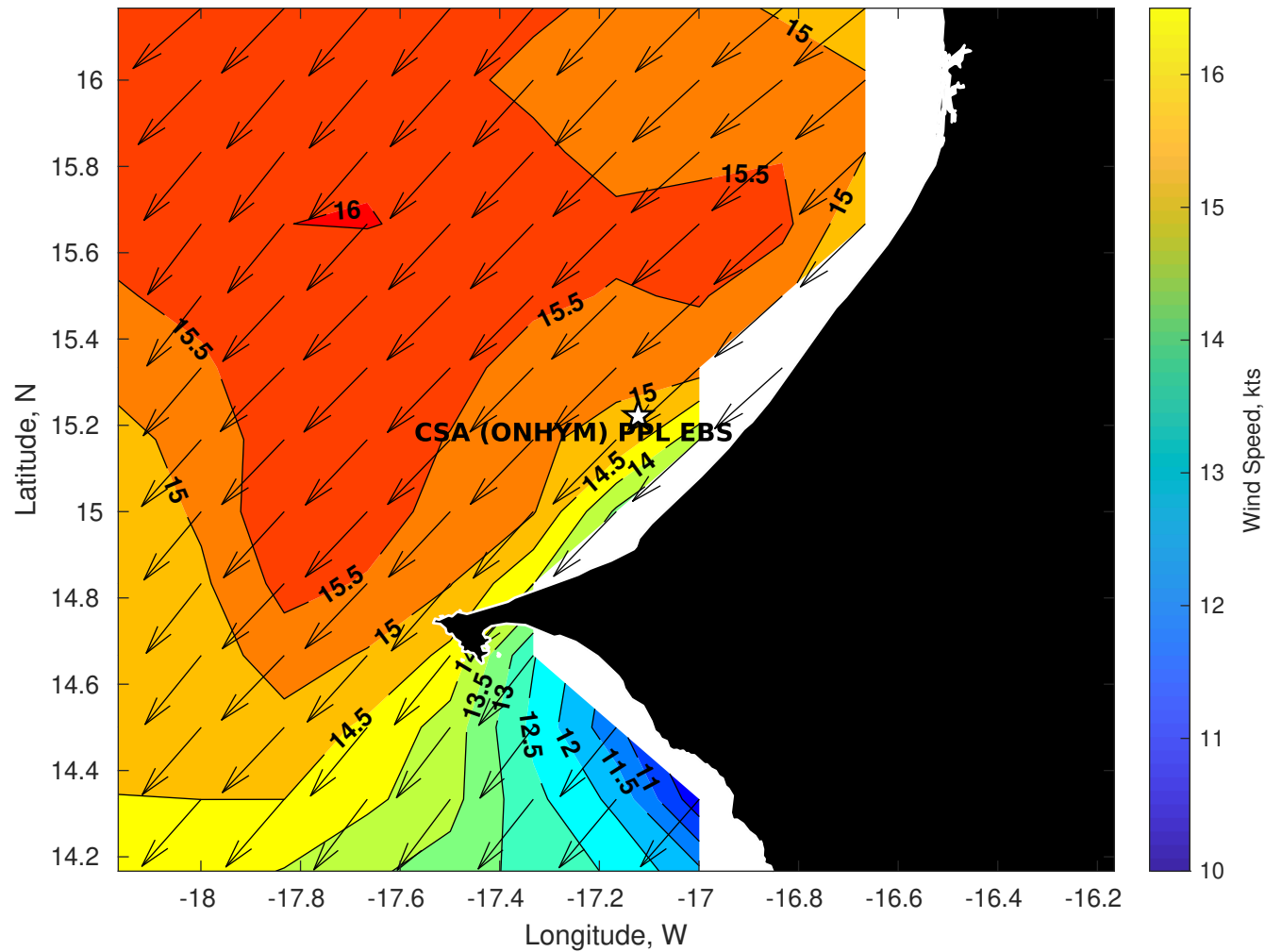
GFS Winds (kts) for CSA (ONHYM) PPL EBS - Senegal at 23-Dec-2025 09:00:00
