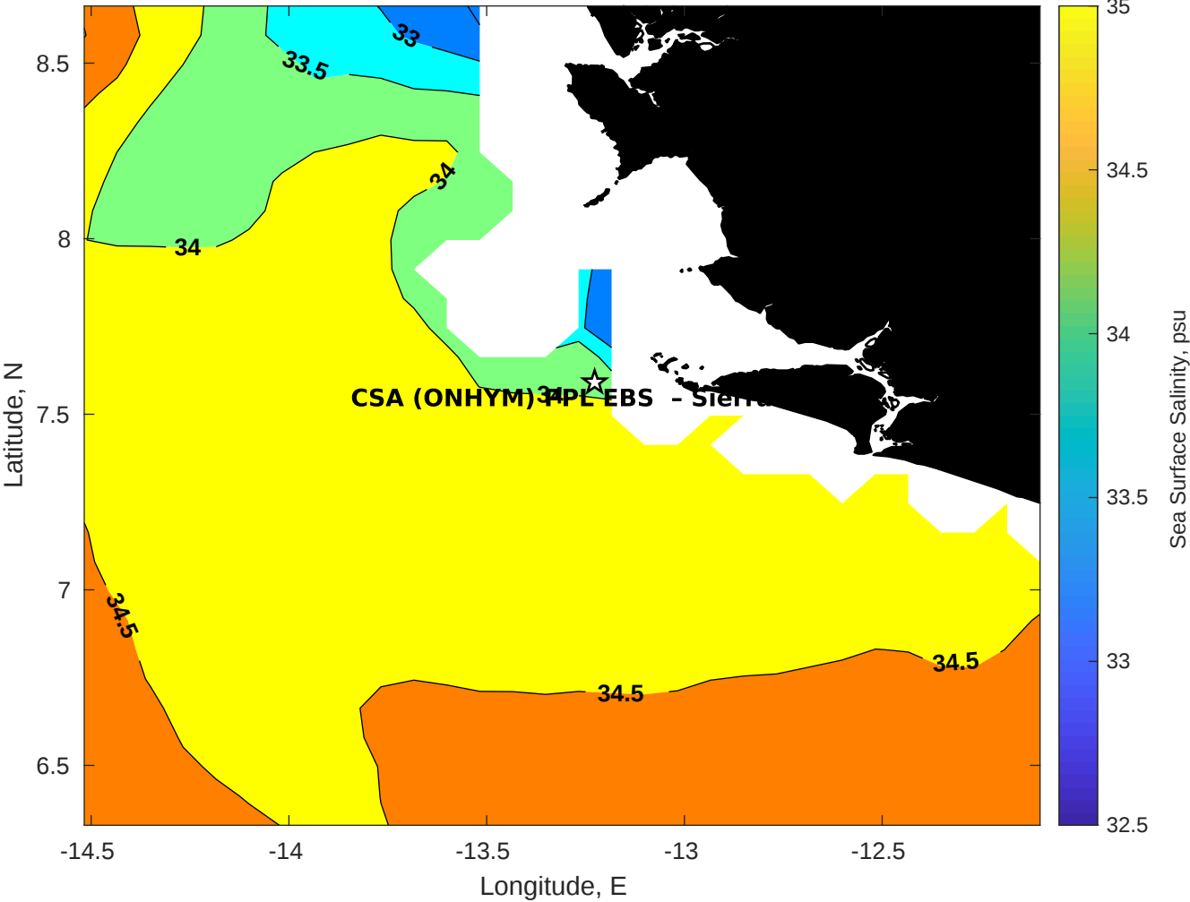
Surface Salinity for CSA (ONHYM) PPL EBS - Sierra Leone at 22-Dec-2025 00:00:00
