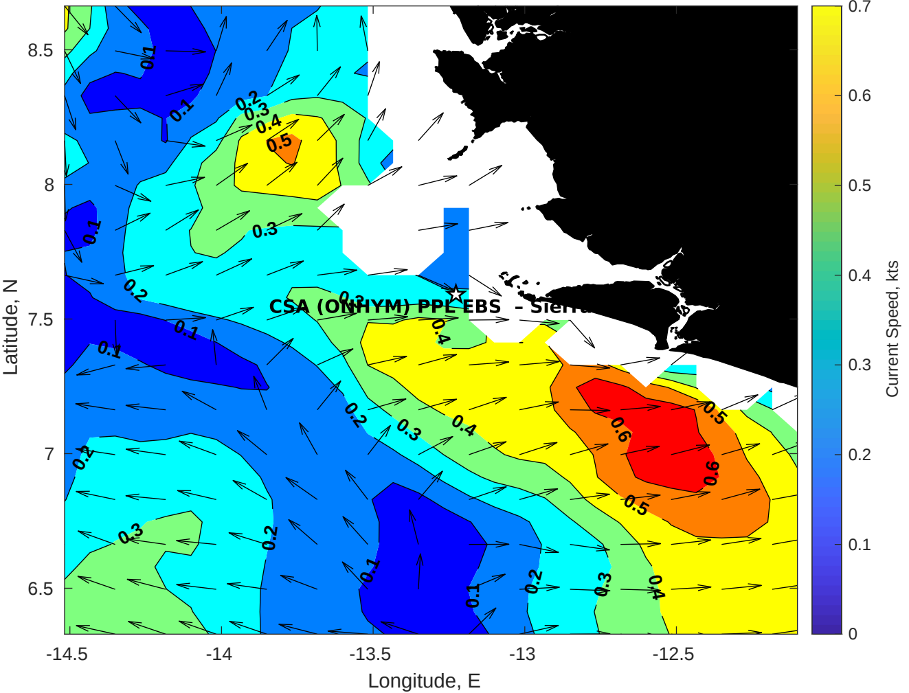
Surface Currents for CSA (ONHYM) PPL EBS - Sierra Leone at 22-Dec-2025 00:00:00
