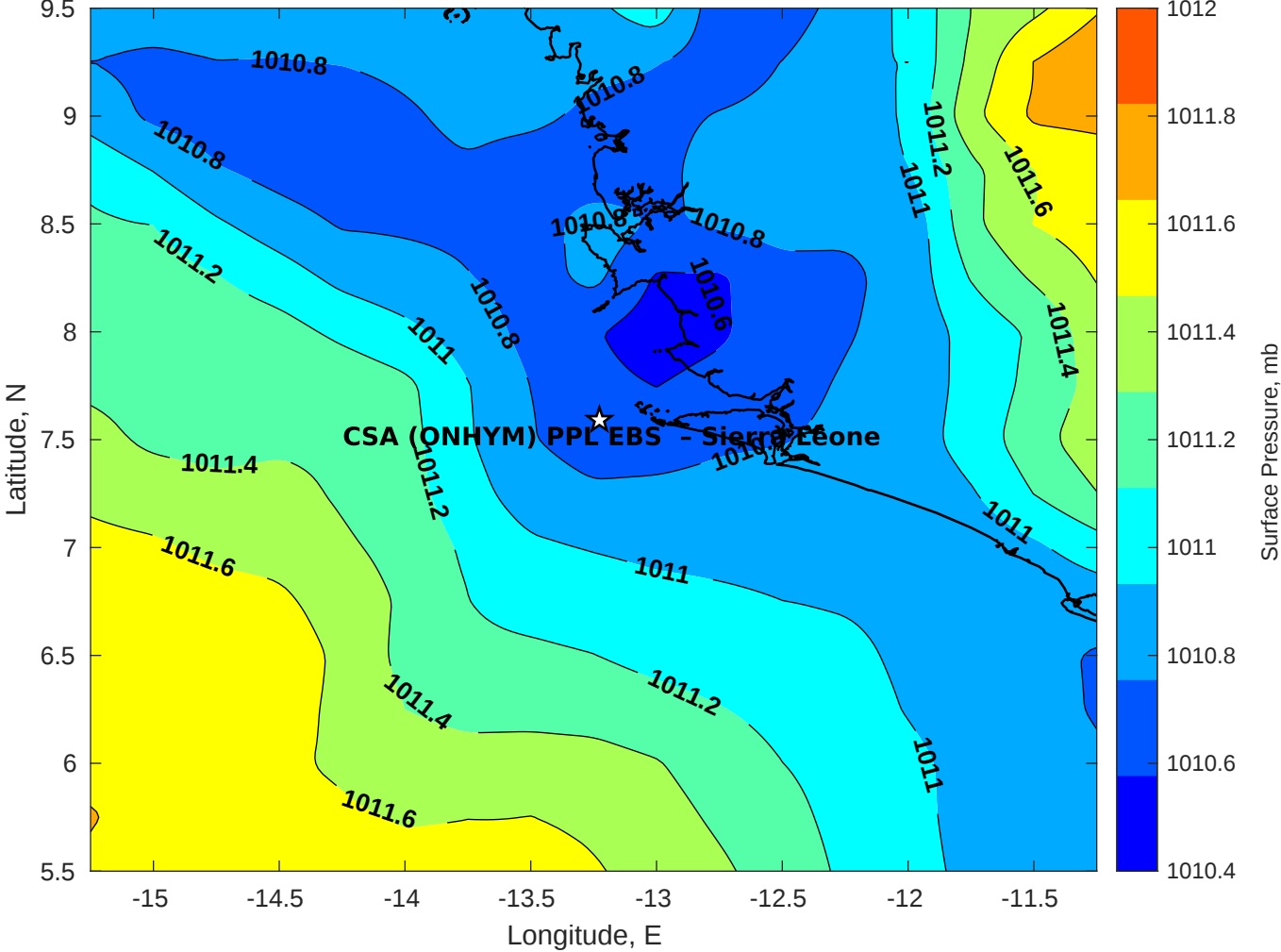
Surface Pressure (mb) for CSA (ONHYM) PPL EBS - Sierra Leone at 23-Dec-2025 00:00:00
