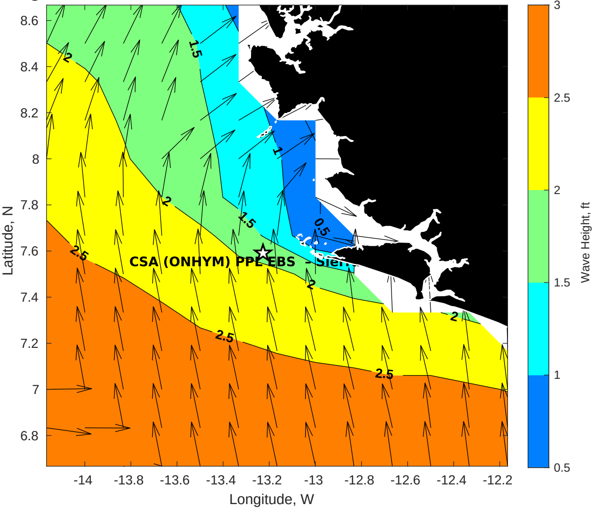
GFS Wave Height (ft) for CSA (ONHYM) PPL EBS - Sierra Leone at 23-Dec-2025 09:00:00
