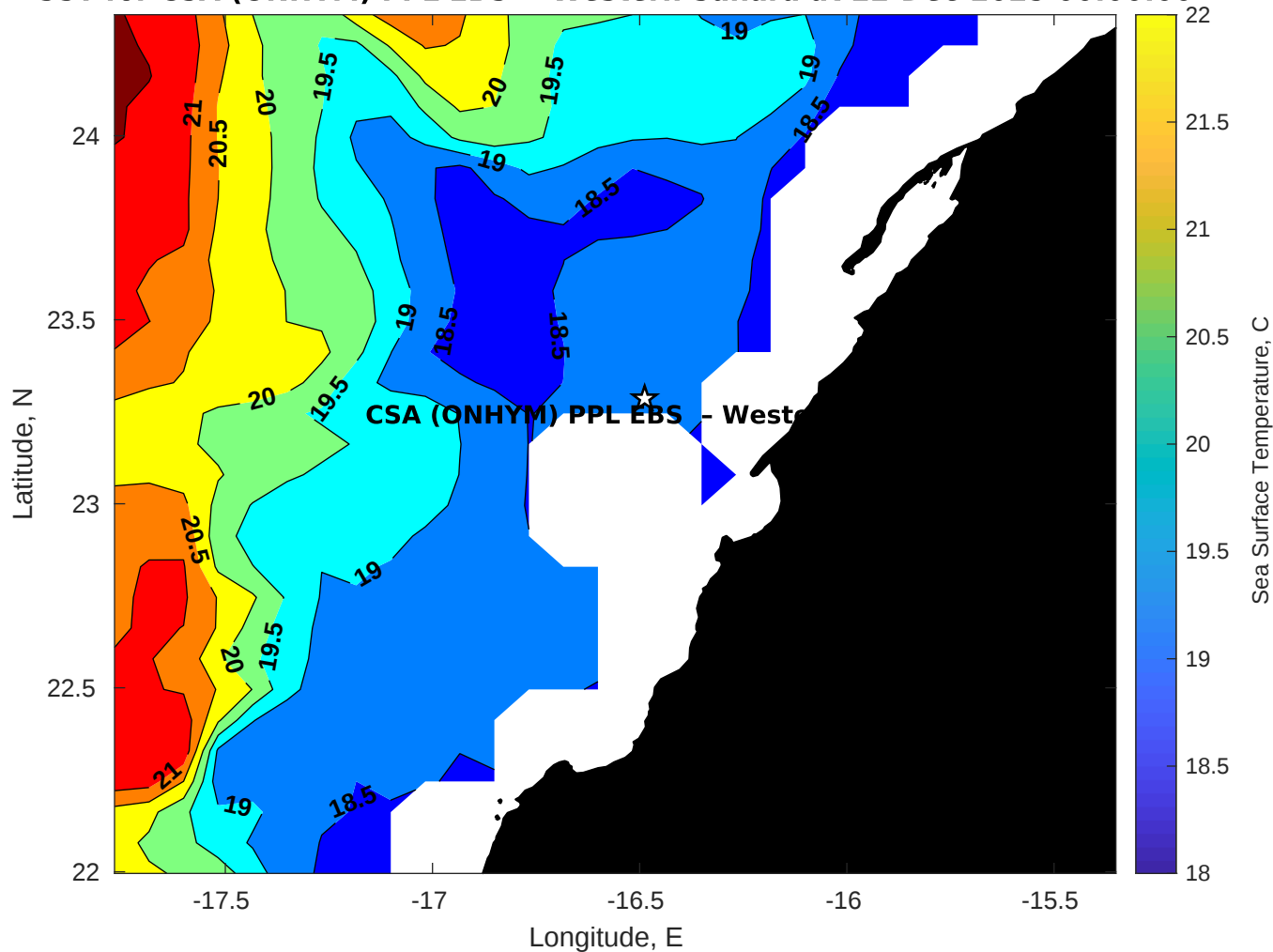
SST for CSA (ONHYM) PPL EBS - Western Sahara at 22-Dec-2025 00:00:00
