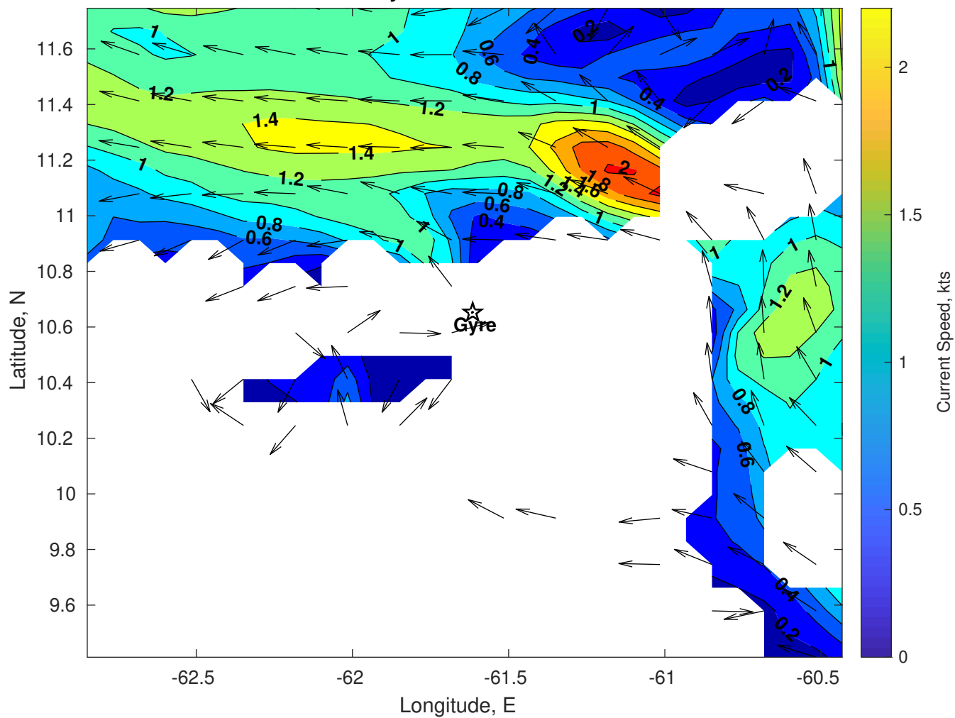
Surface Currents for Gyre at 22-Dec-2025 00:00:00
