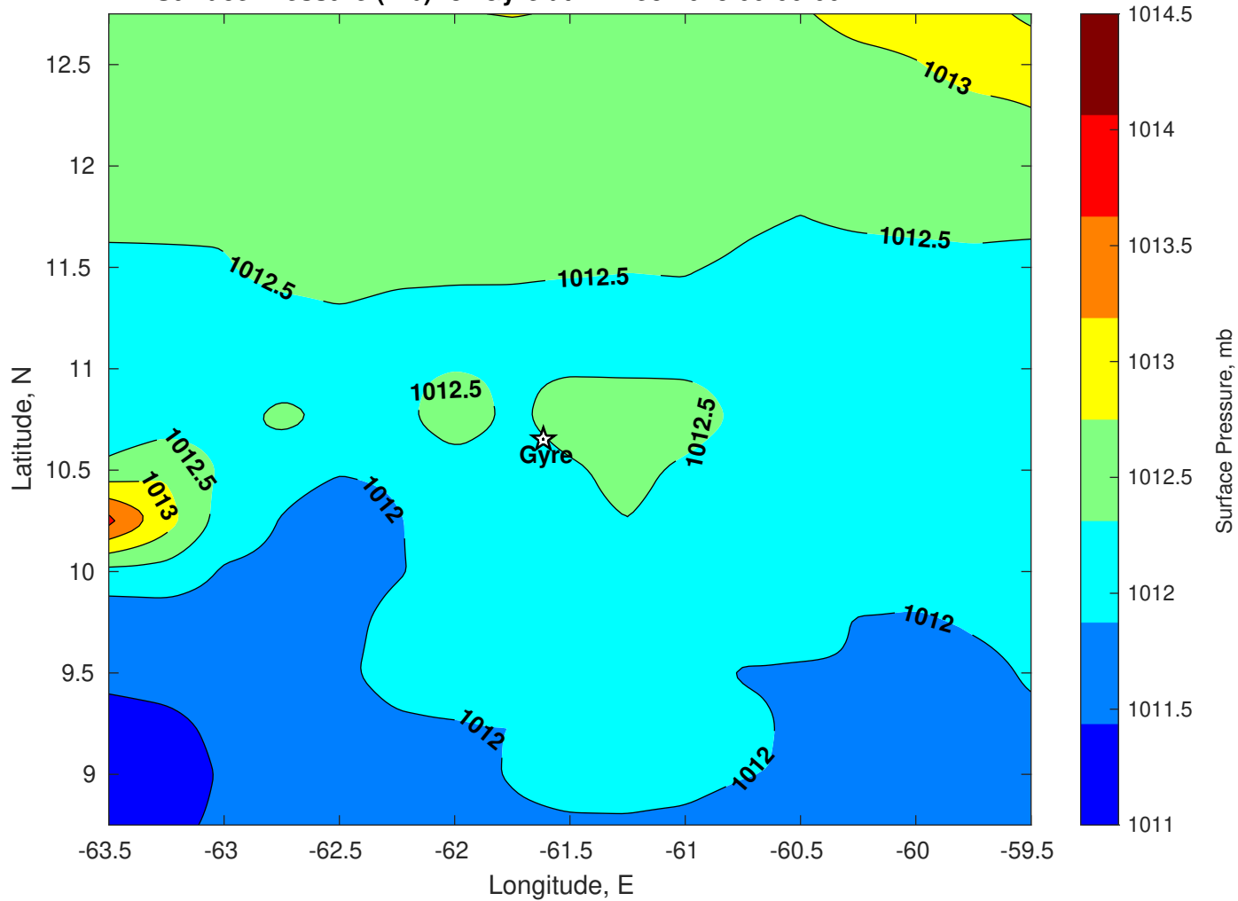
Surface Pressure (mb) for Gyre at 24-Dec-2025 00:00:00
