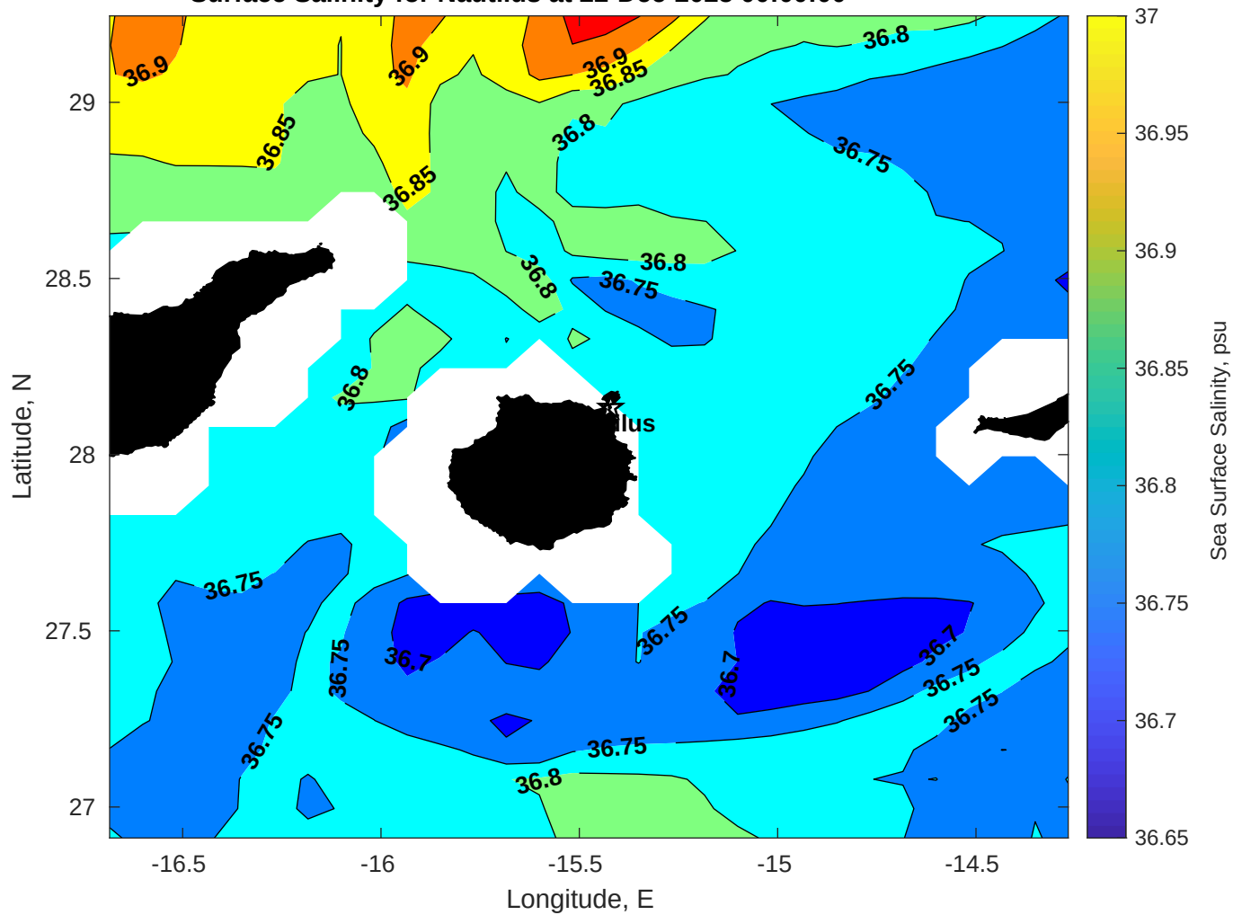
Surface Salinity for Nautilus at 22-Dec-2025 00:00:00
