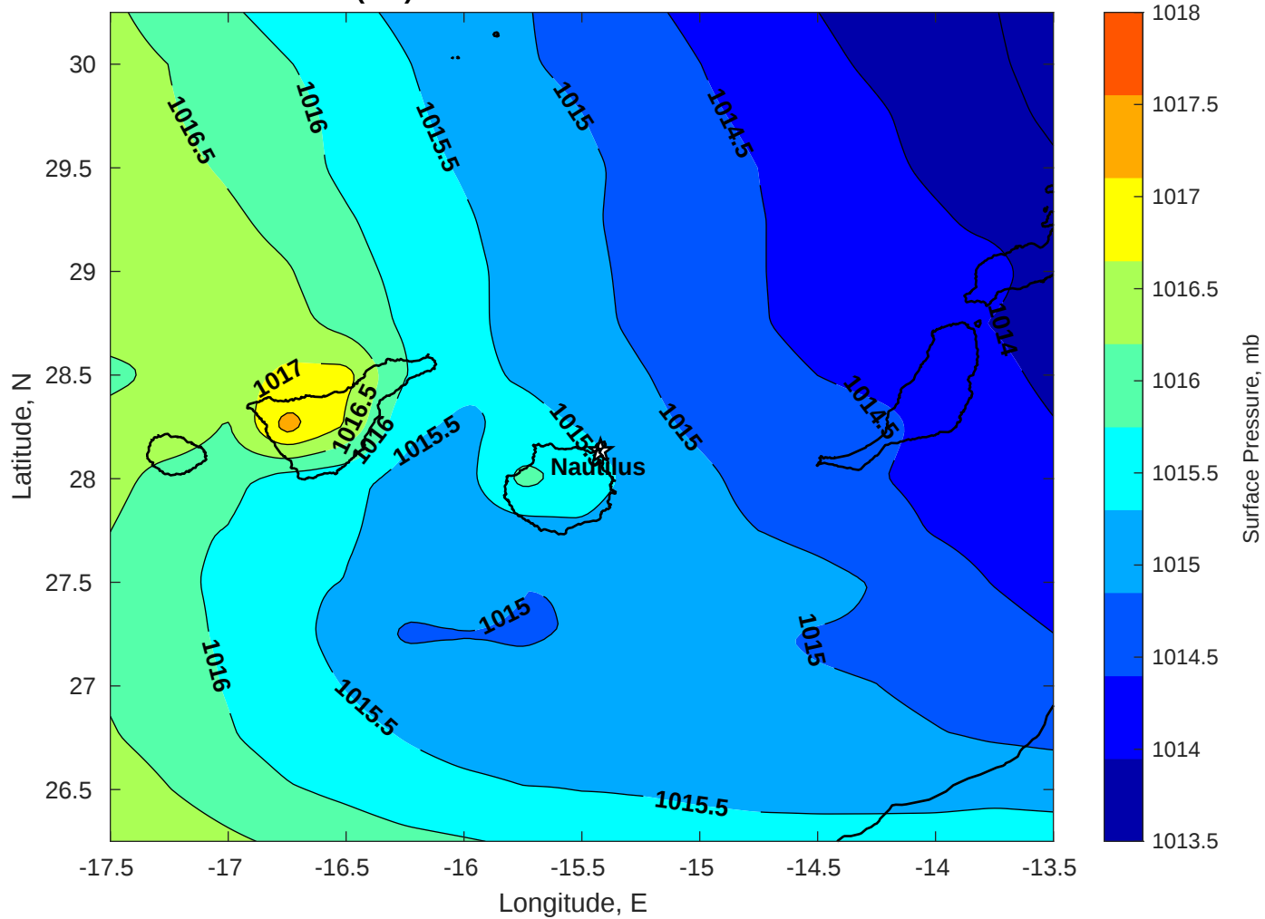
Surface Pressure (mb) for Nautilus at 25-Dec-2025 00:00:00
