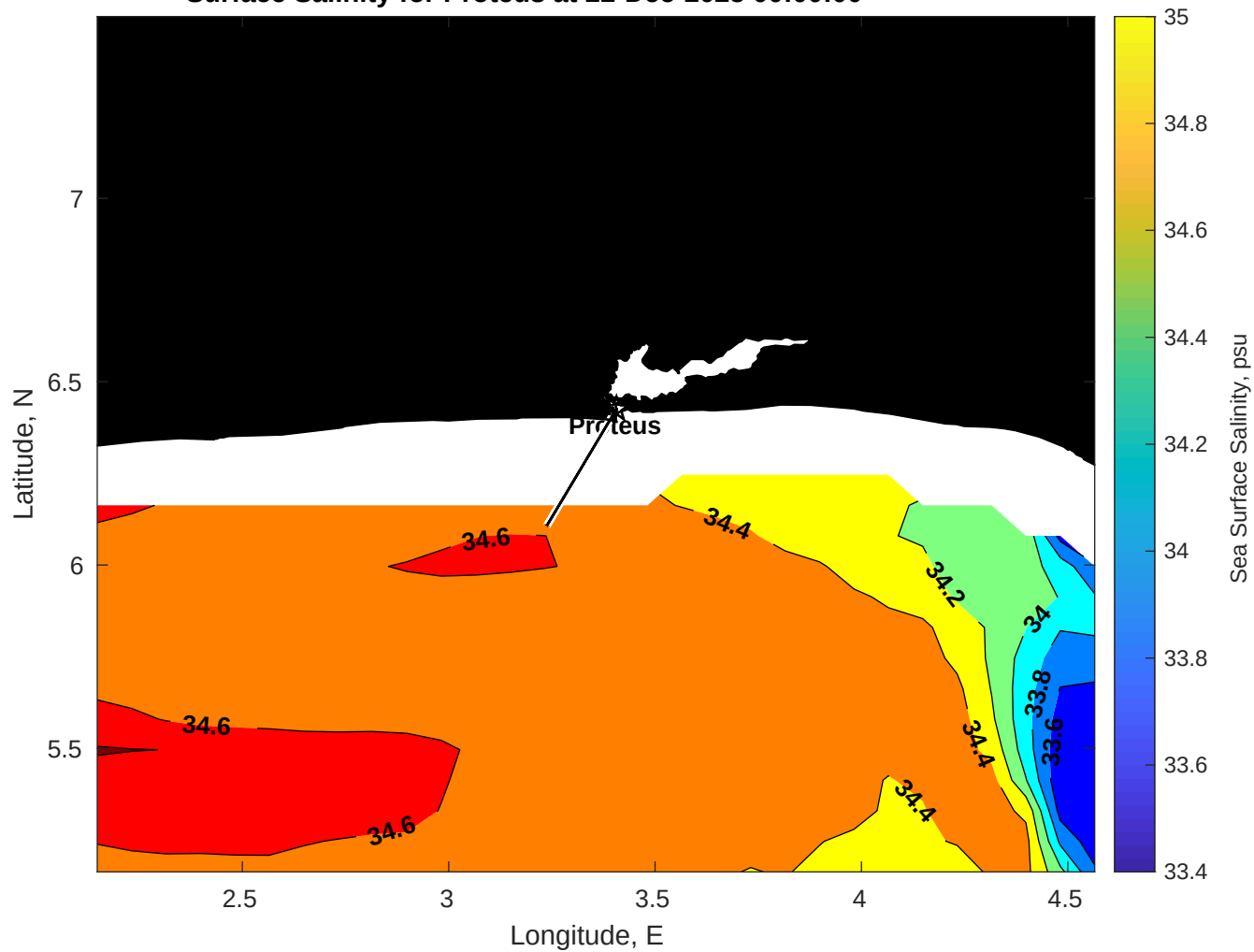
Surface Salinity for Proteus at 22-Dec-2025 00:00:00
