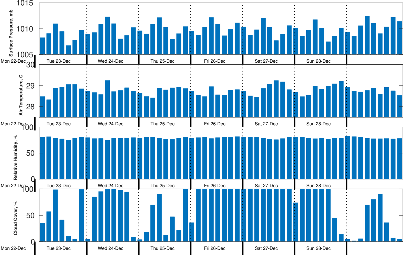
Met Forecast for Proteus from 23-Dec-2025 00:00:00 to 30-Dec-2025 00:00:00
