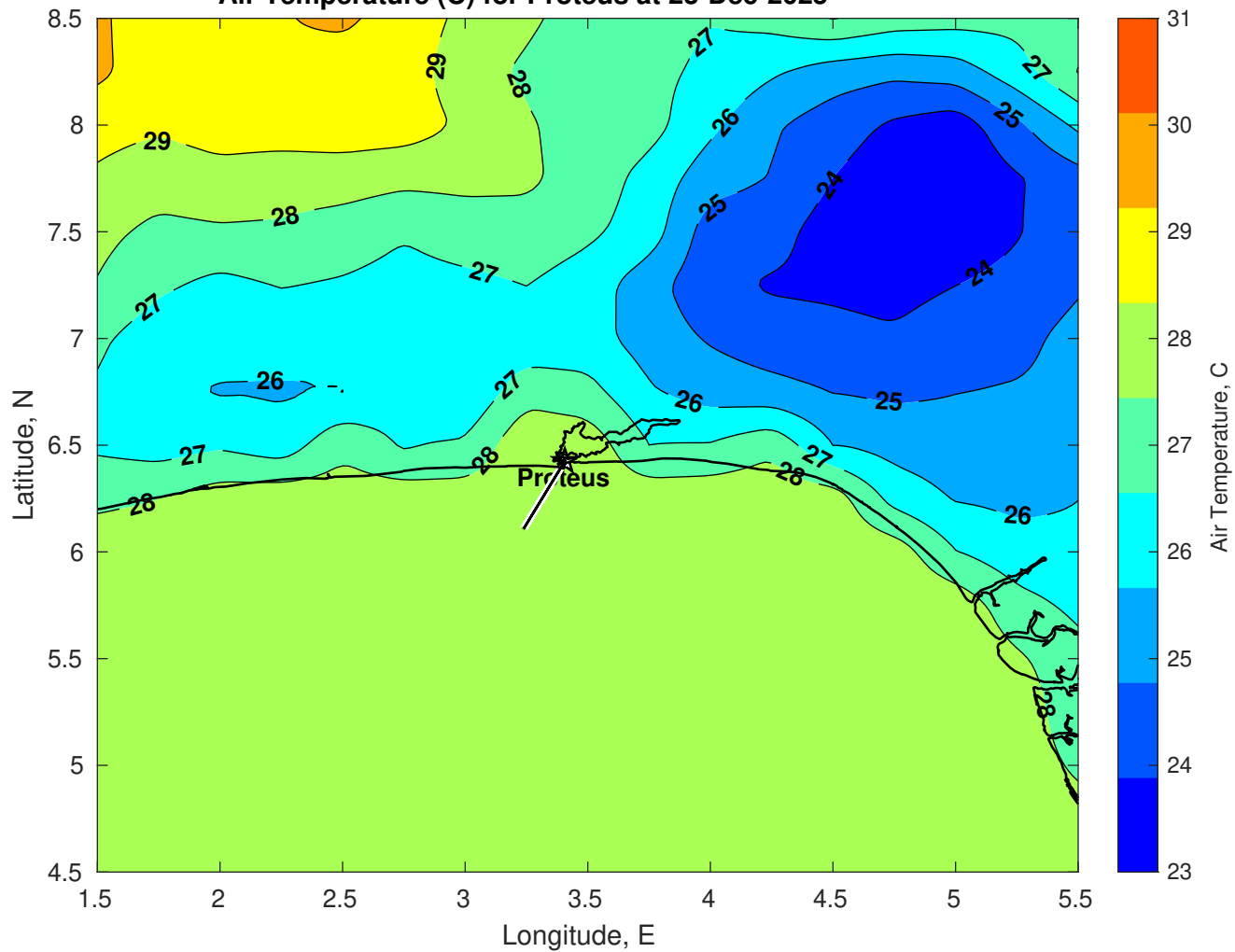
Air Temperature (C) for Proteus at 23-Dec-2025
