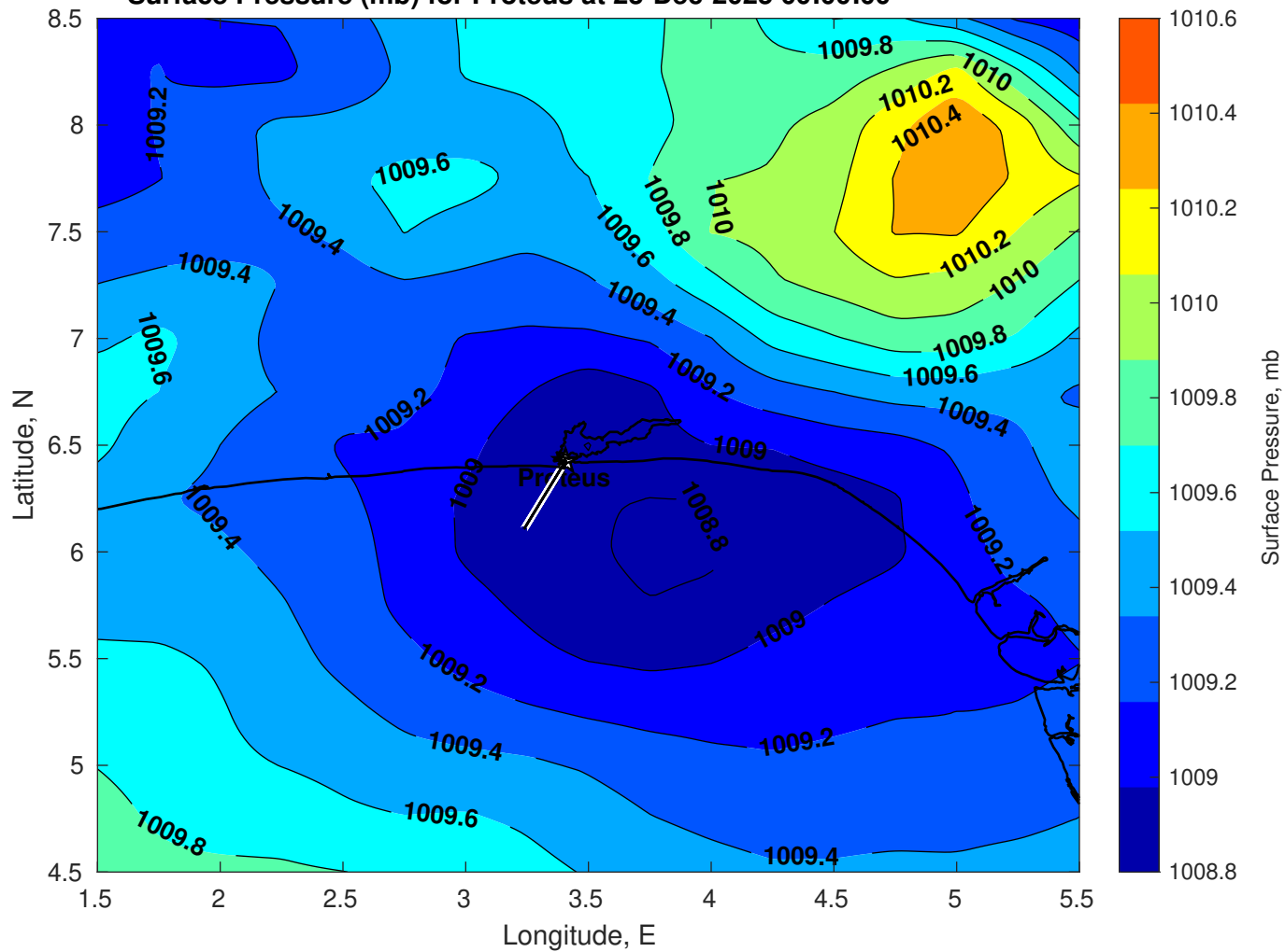
Surface Pressure (mb) for Proteus at 23-Dec-2025 00:00:00
