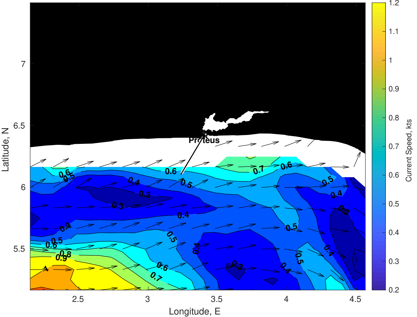
Surface Currents for Proteus at 22-Dec-2025 00:00:00
