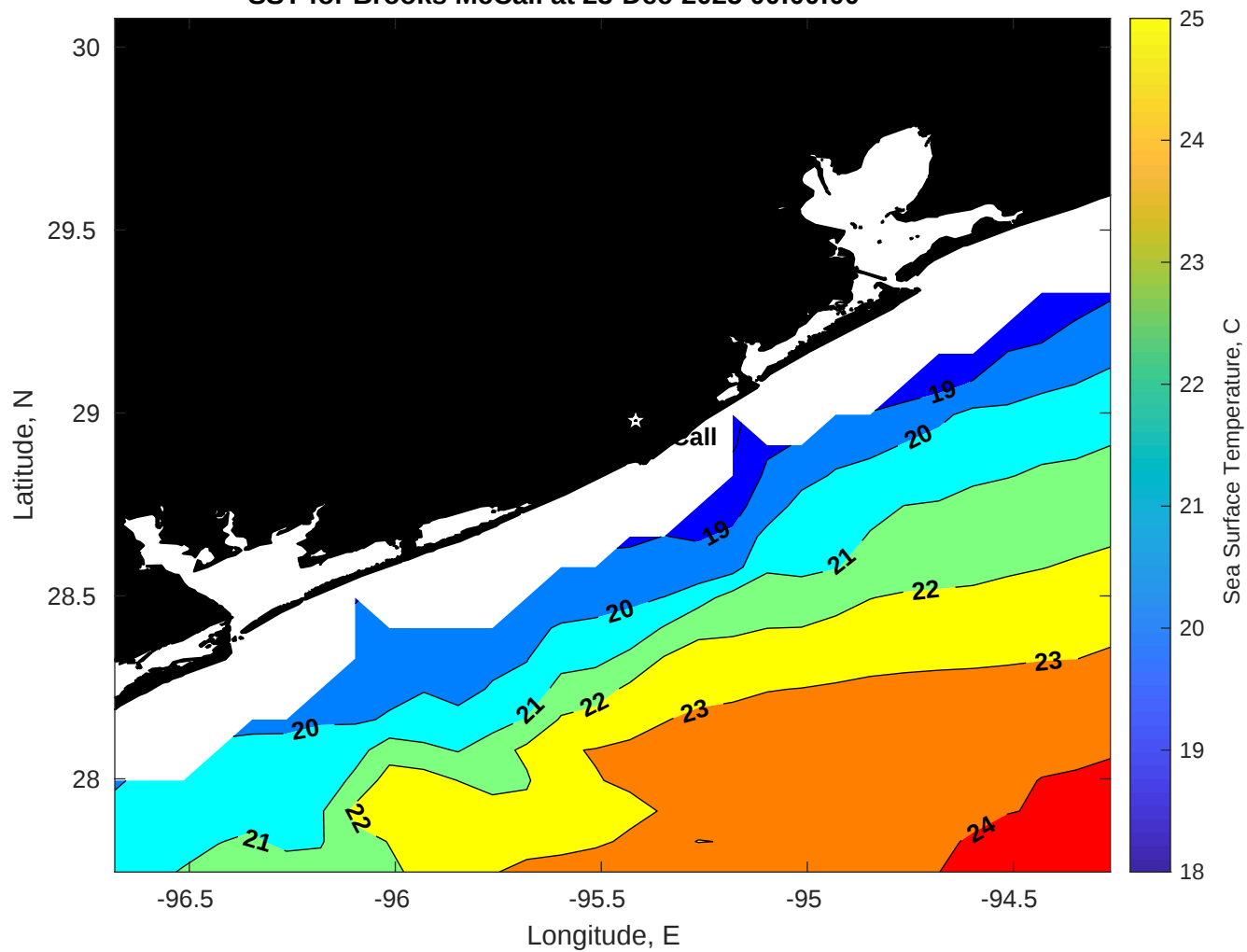
SST for Brooks McCall at 23-Dec-2025 00:00:00
