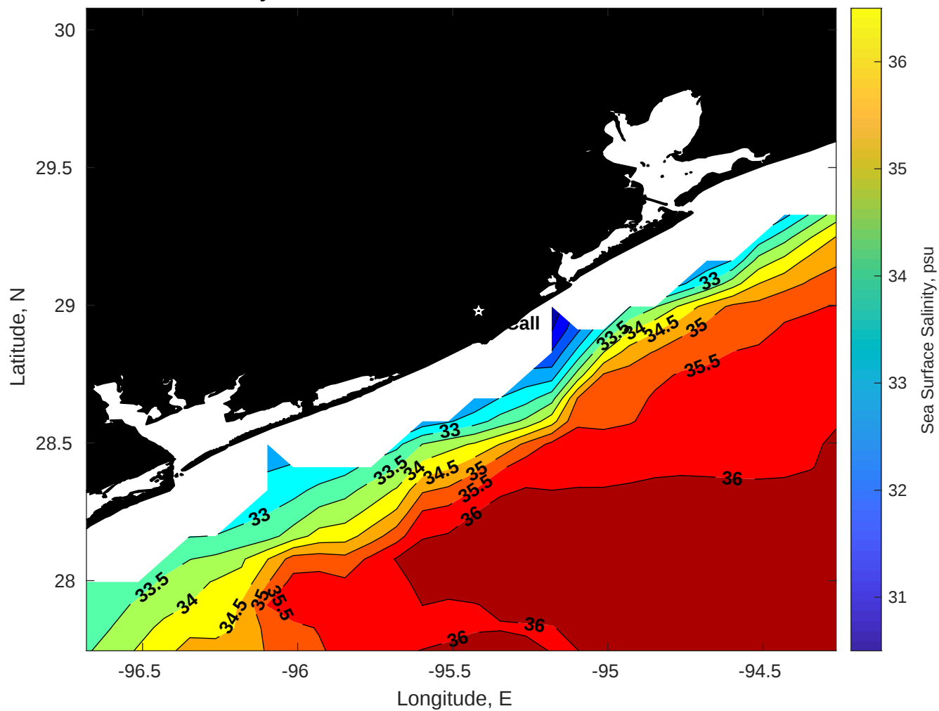
Surface Salinity for Brooks McCall at 23-Dec-2025 00:00:00
