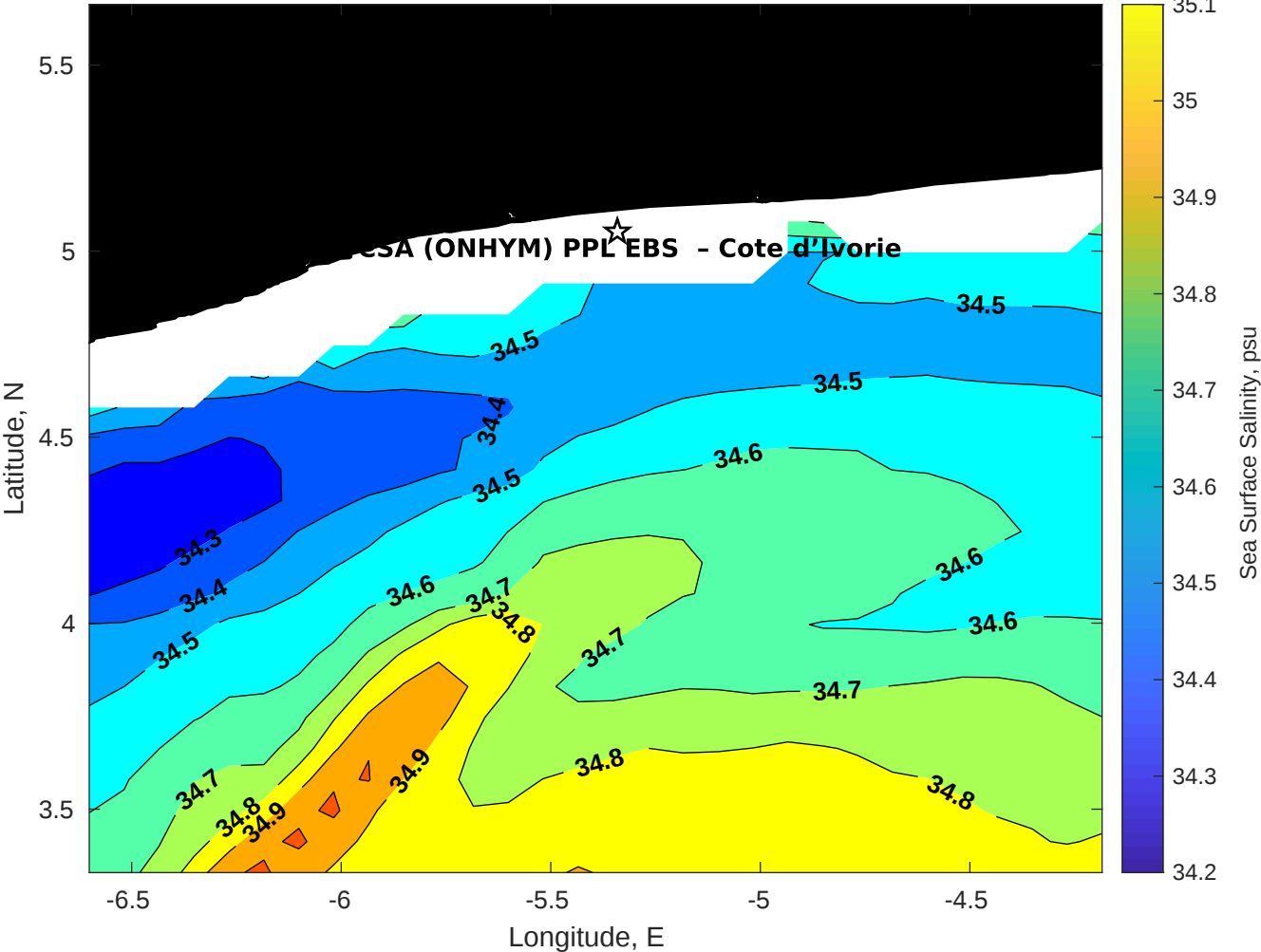
Surface Salinity for CSA (ONHYM) PPL EBS - Cote d'Ivoire at 23-Dec-2025 00:00:00
