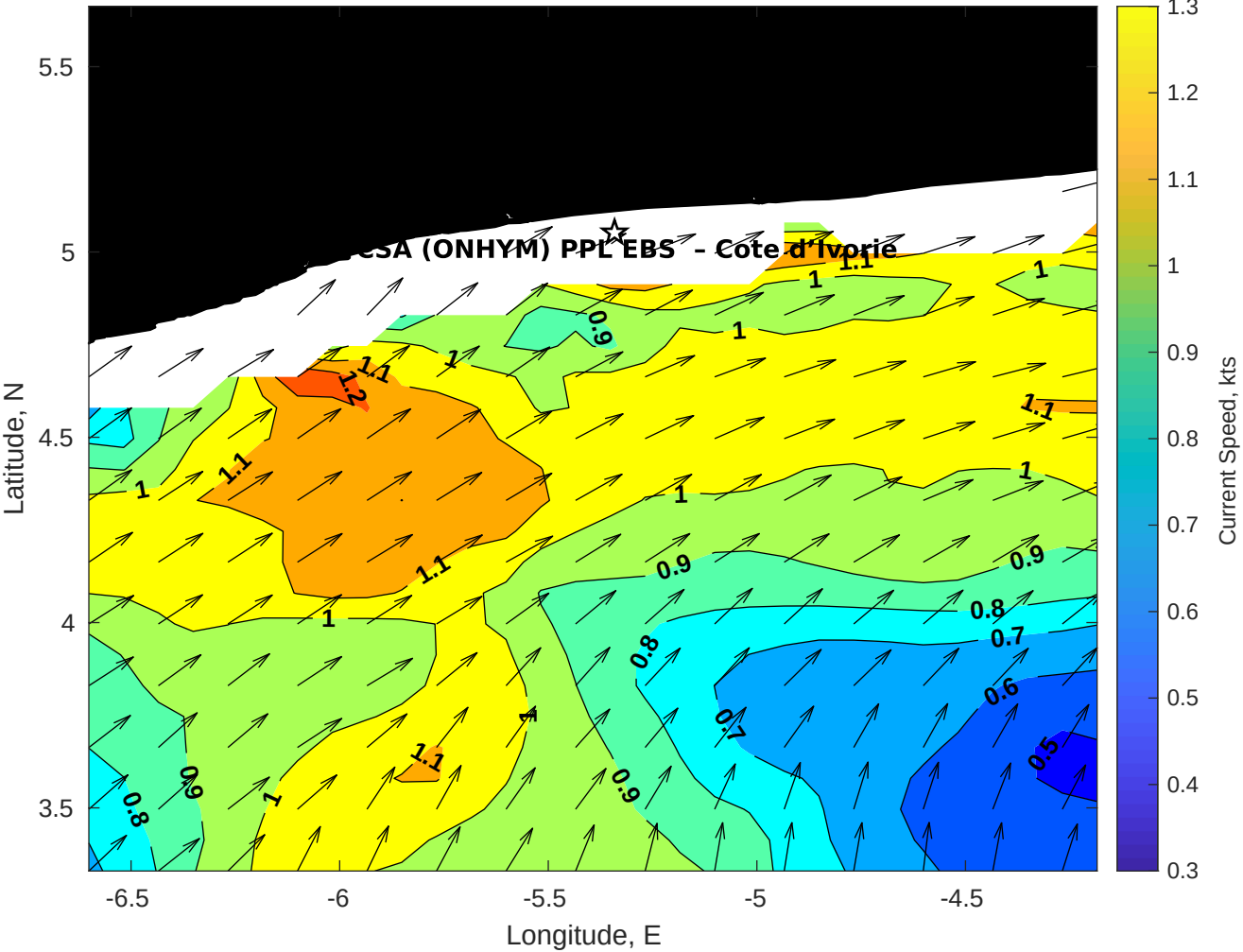
Surface Currents for CSA (ONHYM) PPL EBS - Cote d'Ivoire at 23-Dec-2025 00:00:00
