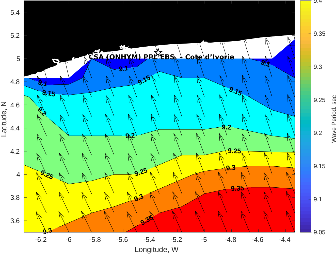
GFS Wave Period (sec) for CSA (ONHYM) PPL EBS - Cote d'Ivoire at 24-Dec-2025 09:00:00
