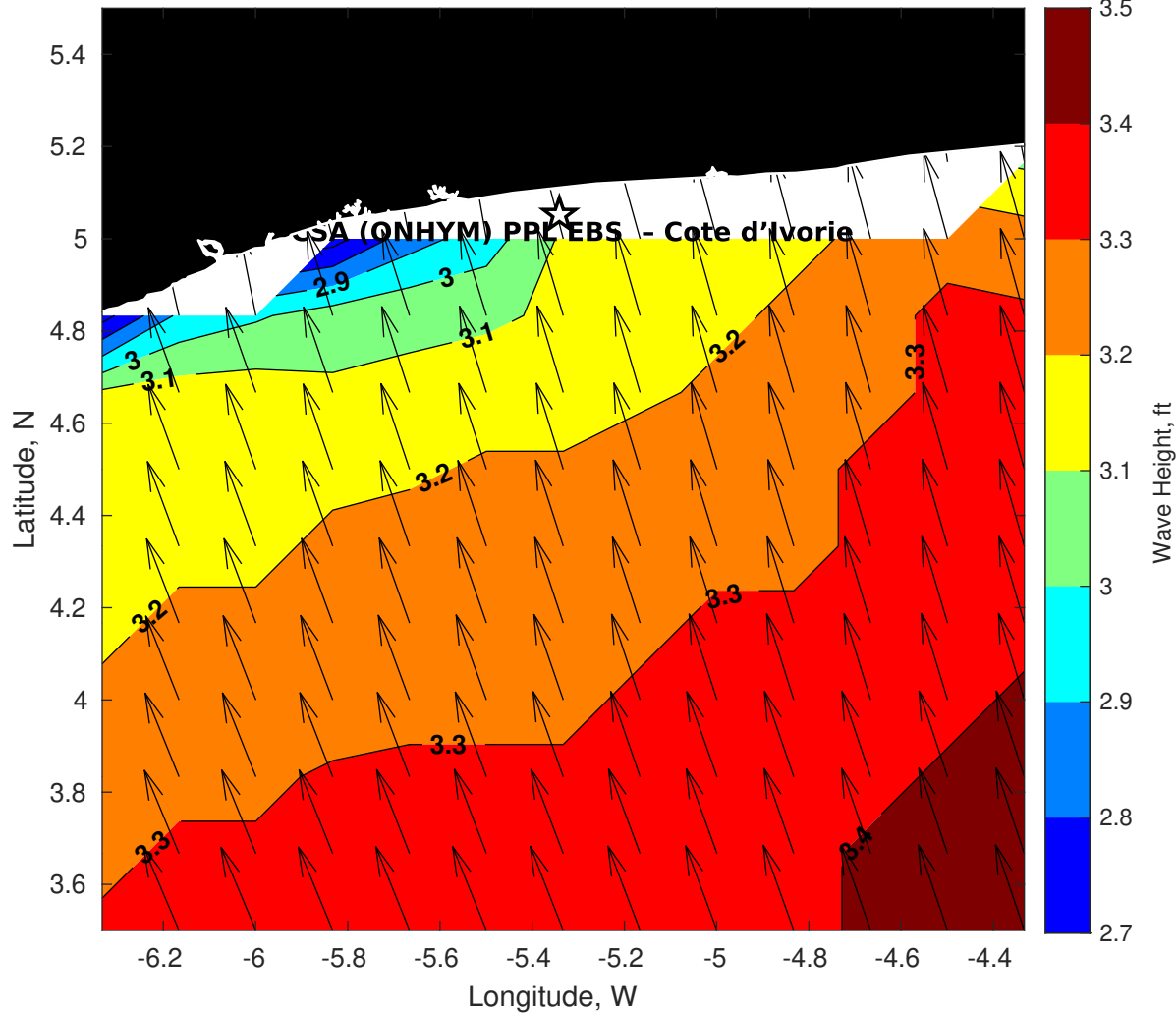
GFS Wave Height (ft) for CSA (ONHYM) PPL EBS - Cote d'Ivoire at 24-Dec-2025 09:00:00
