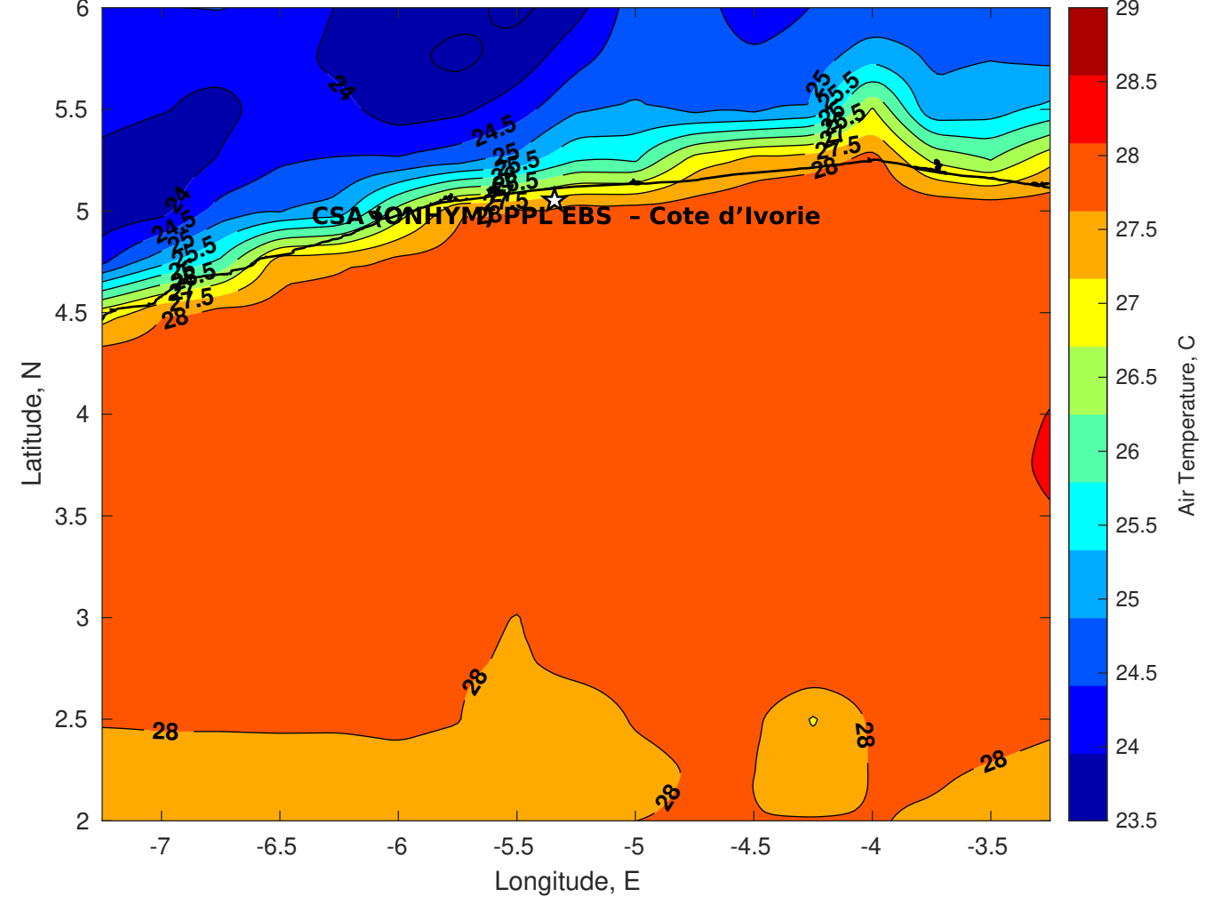
Air Temperature (C) for CSA (ONHYM) PPL EBS - Cote d'Ivoire at 24-Dec-2025
