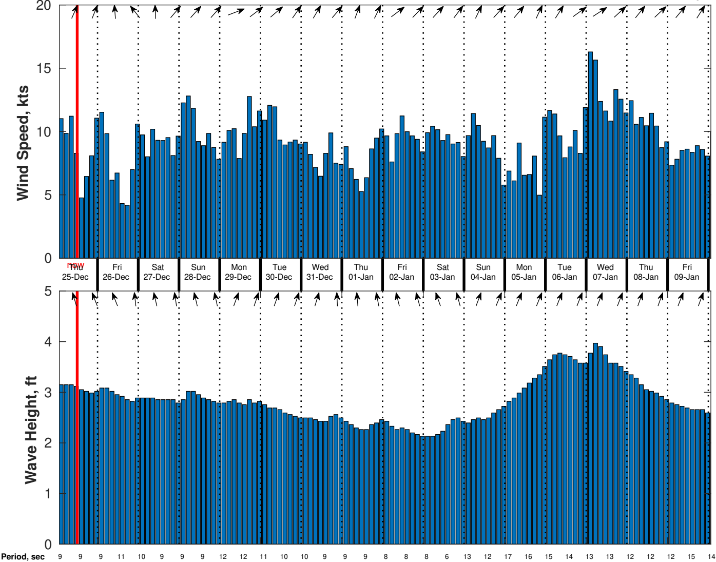
Wind & Wave Forecast for CSA (ONHYM) PPL EBS - Cote d'Ivoire from 24-Dec-2025 01:00:00 to 09-Jan-2026 01:00:00
