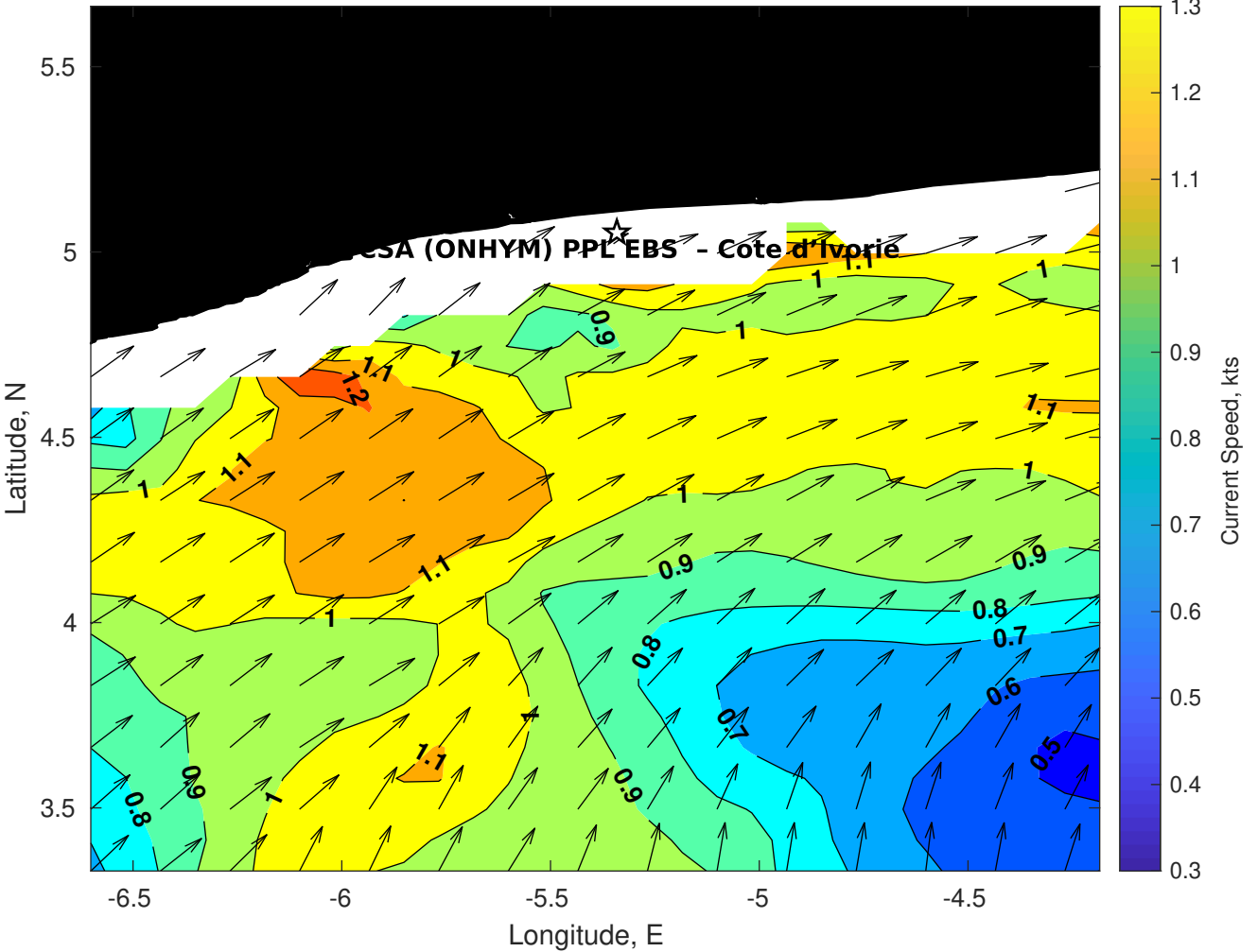
Surface Currents for CSA (ONHYM) PPL EBS - Cote d'Ivoire at 23-Dec-2025 00:00:00
