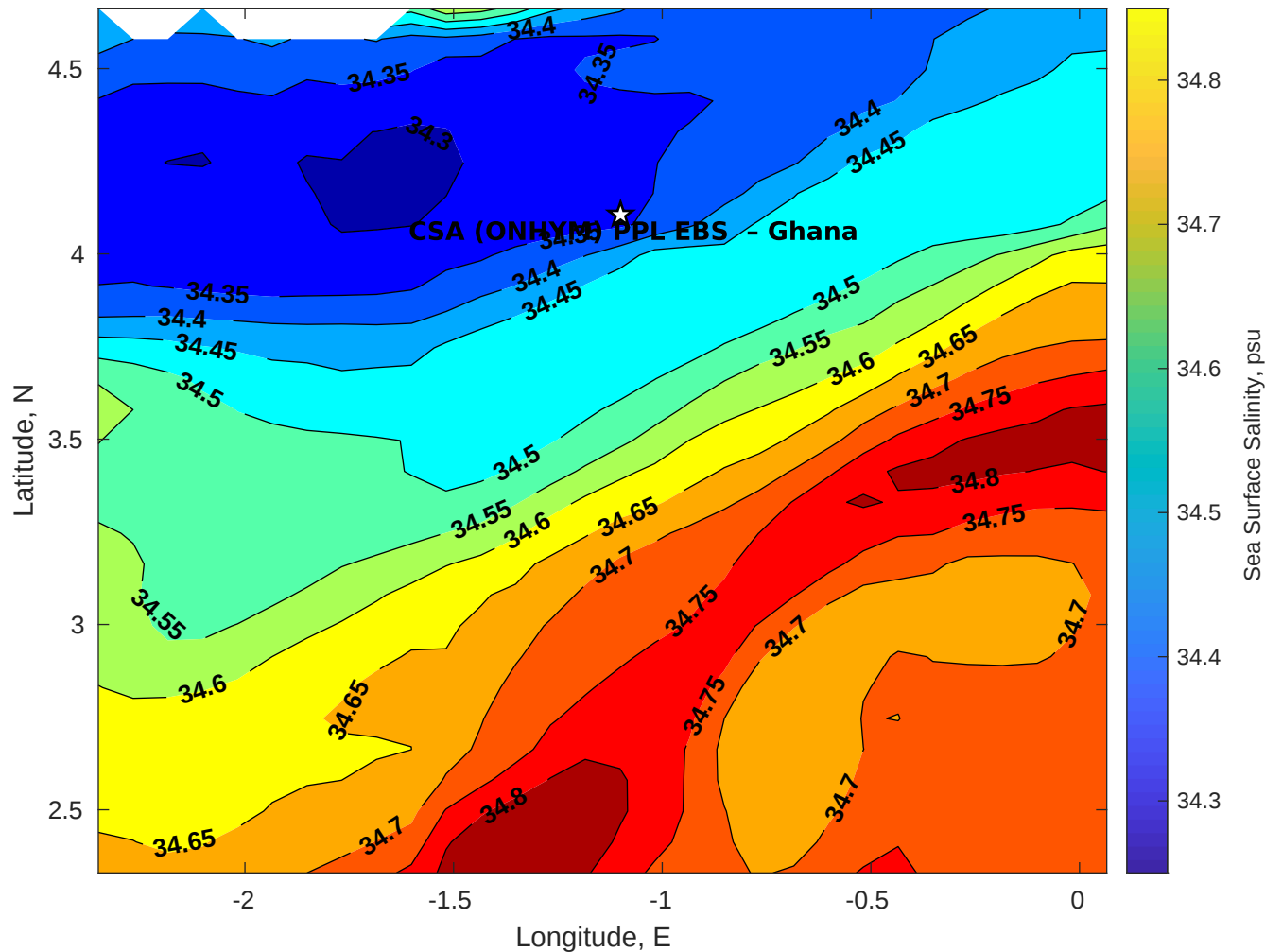
Surface Salinity for CSA (ONHYM) PPL EBS - Ghana at 23-Dec-2025 00:00:00
