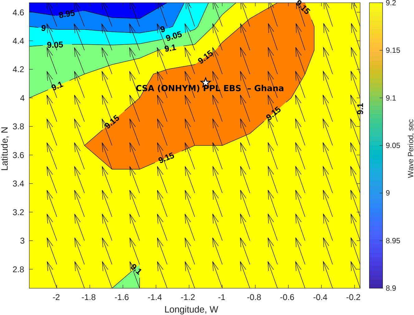
GFS Wave Period (sec) for CSA (ONHYM) PPL EBS - Ghana at 24-Dec-2025 09:00:00
