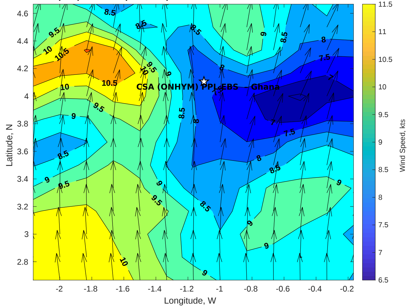
GFS Winds (kts) for CSA (ONHYM) PPL EBS - Ghana at 24-Dec-2025 09:00:00
