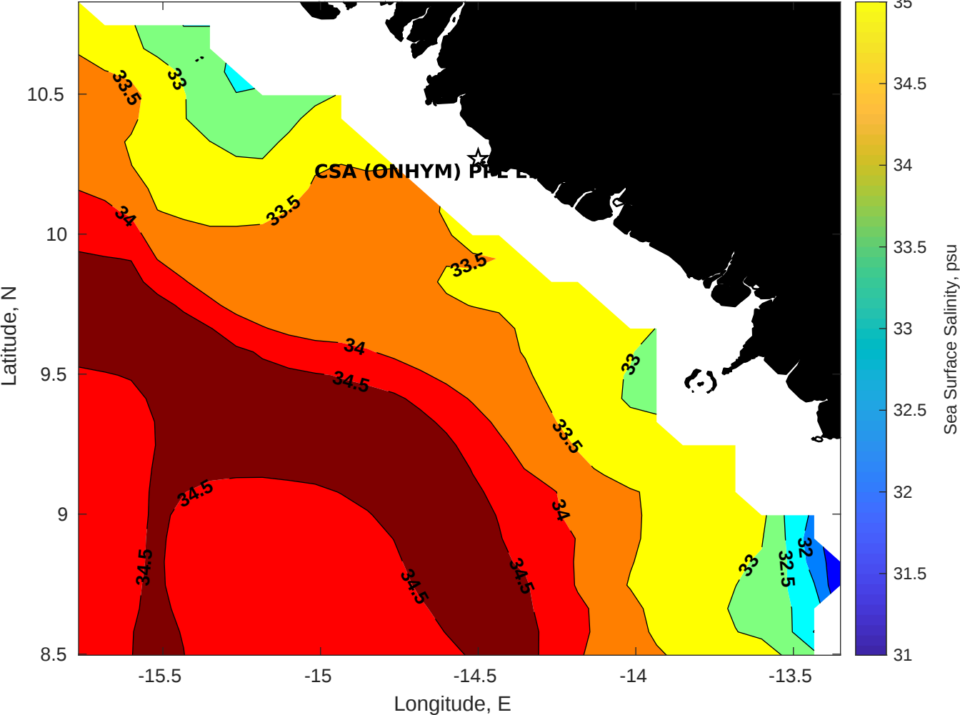
Surface Salinity for CSA (ONHYM) PPL EBS - Guinea at 23-Dec-2025 00:00:00
