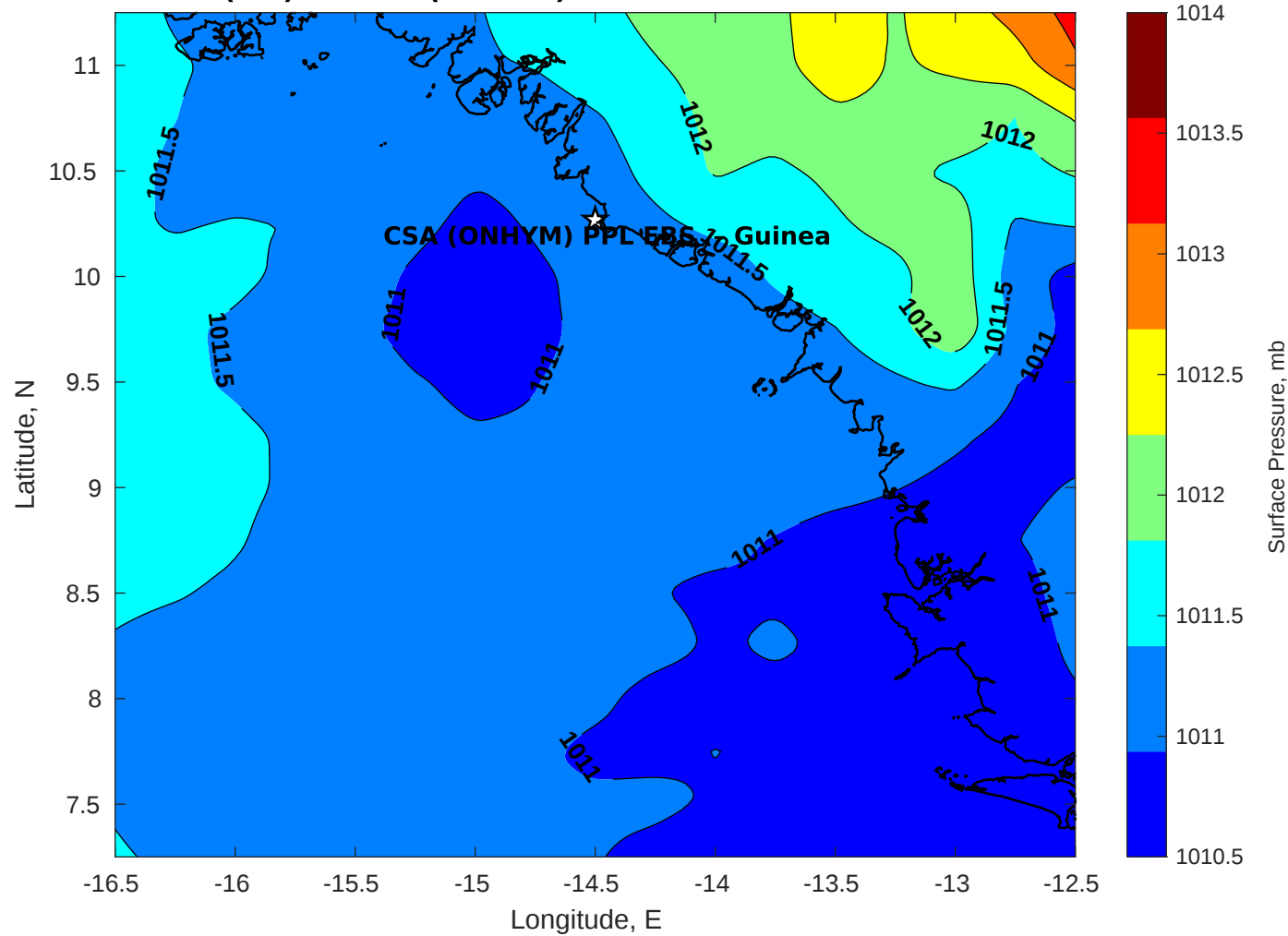
Surface Pressure (mb) for CSA (ONHYM) PPL EBS - Guinea at 25-Dec-2025 00:00:00
