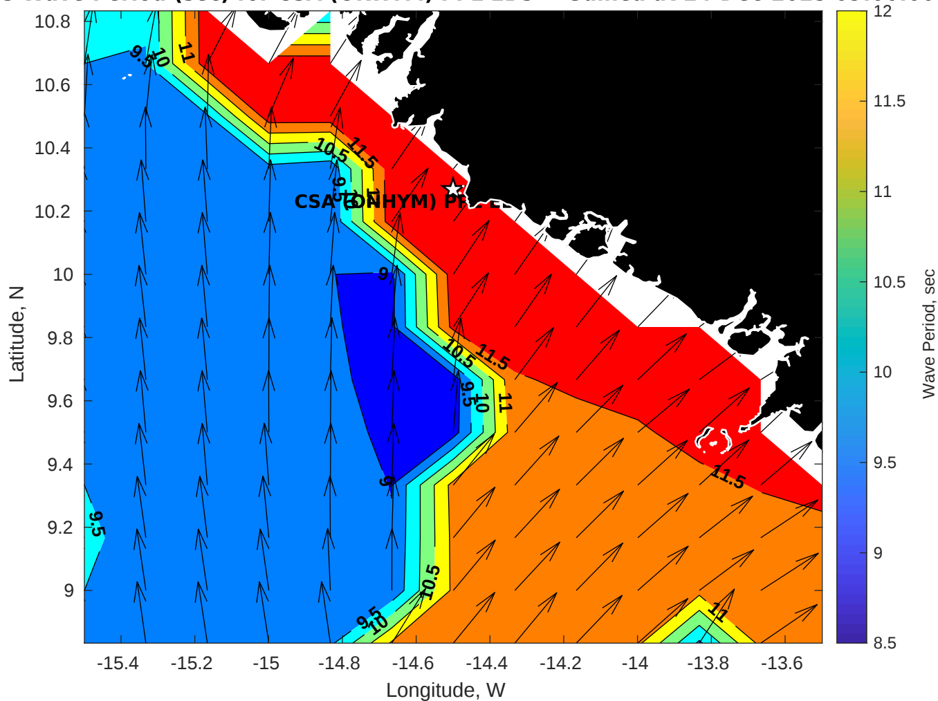
GFS Wave Period (sec) for CSA (ONHYM) PPL EBS - Guinea at 24-Dec-2025 09:00:00
