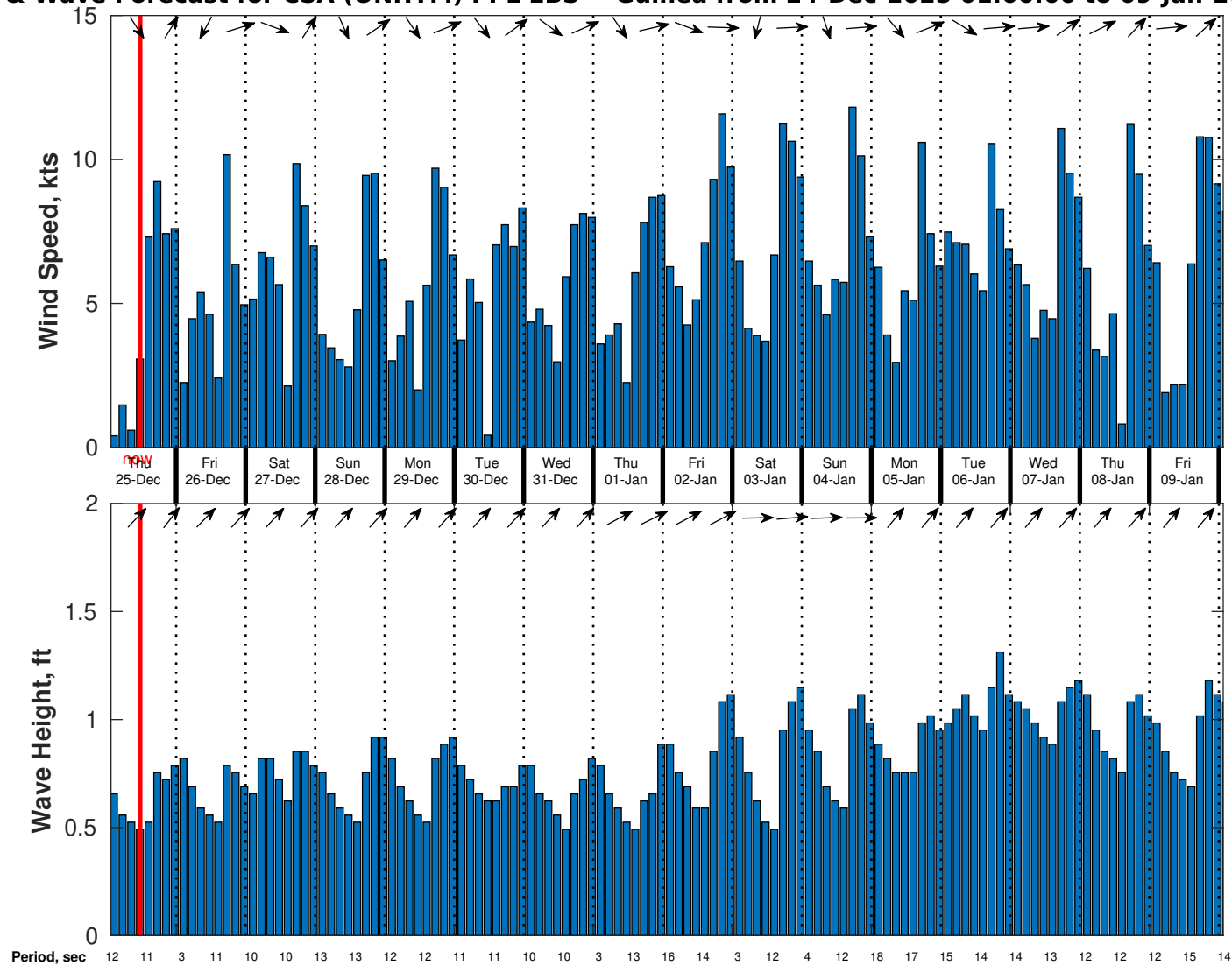
Wind & Wave Forecast for CSA (ONHYM) PPL EBS - Guinea from 24-Dec-2025 01:00:00 to 09-Jan-2026 01:00:00
