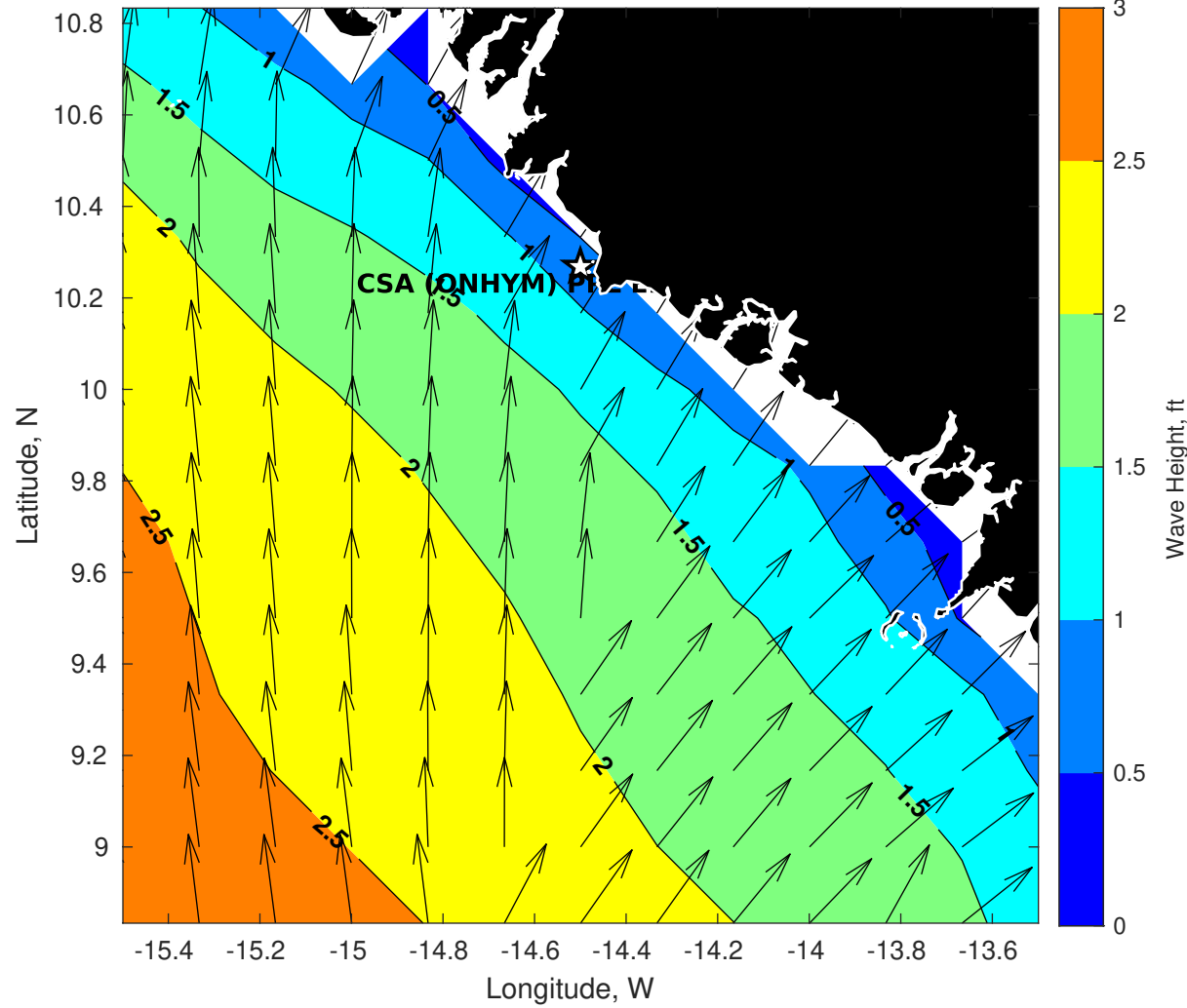
GFS Wave Height (ft) for CSA (ONHYM) PPL EBS - Guinea at 24-Dec-2025 09:00:00
