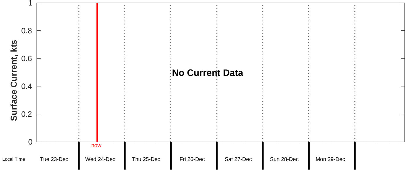
Surface Current Forecast for CSA (ONHYM) PPL EBS - Guinea from 23-Dec-2025 00:00:00 to 31-Dec-2025 00:00:00
