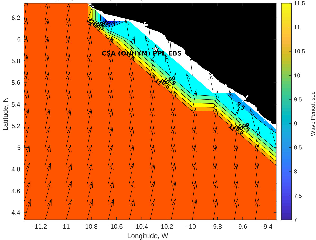
GFS Wave Period (sec) for CSA (ONHYM) PPL EBS - Liberia at 24-Dec-2025 09:00:00
