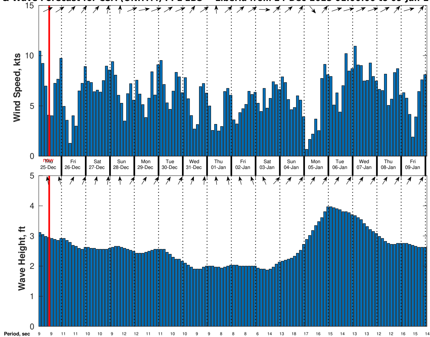
Wind & Wave Forecast for CSA (ONHYM) PPL EBS - Liberia from 24-Dec-2025 01:00:00 to 09-Jan-2026 01:00:00
