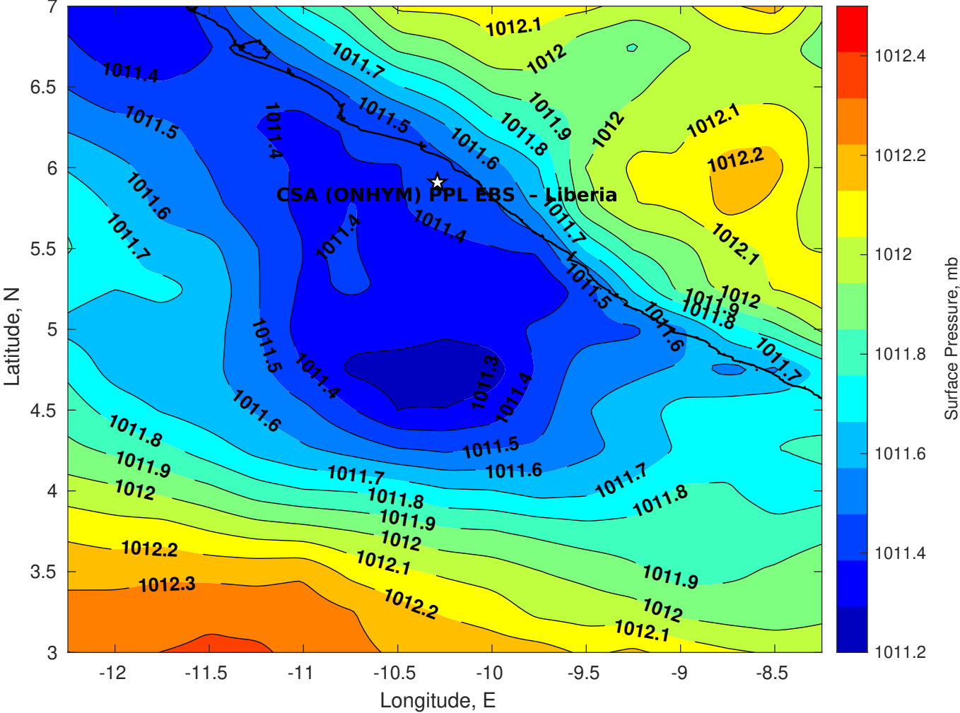
Surface Pressure (mb) for CSA (ONHYM) PPL EBS - Liberia at 24-Dec-2025 00:00:00
