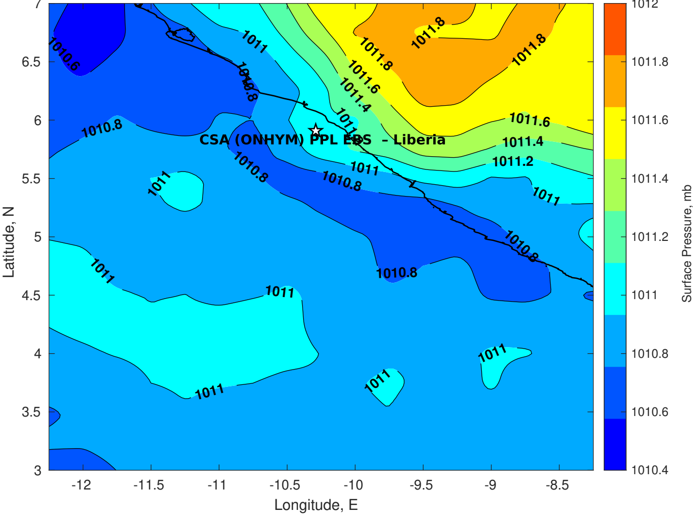
Surface Pressure (mb) for CSA (ONHYM) PPL EBS - Liberia at 25-Dec-2025 00:00:00
