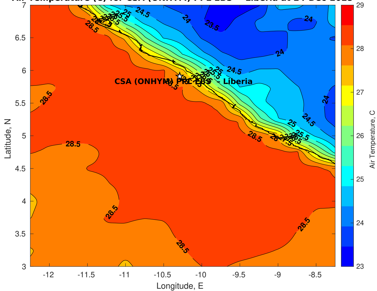
Air Temperature (C) for CSA (ONHYM) PPL EBS - Liberia at 24-Dec-2025
