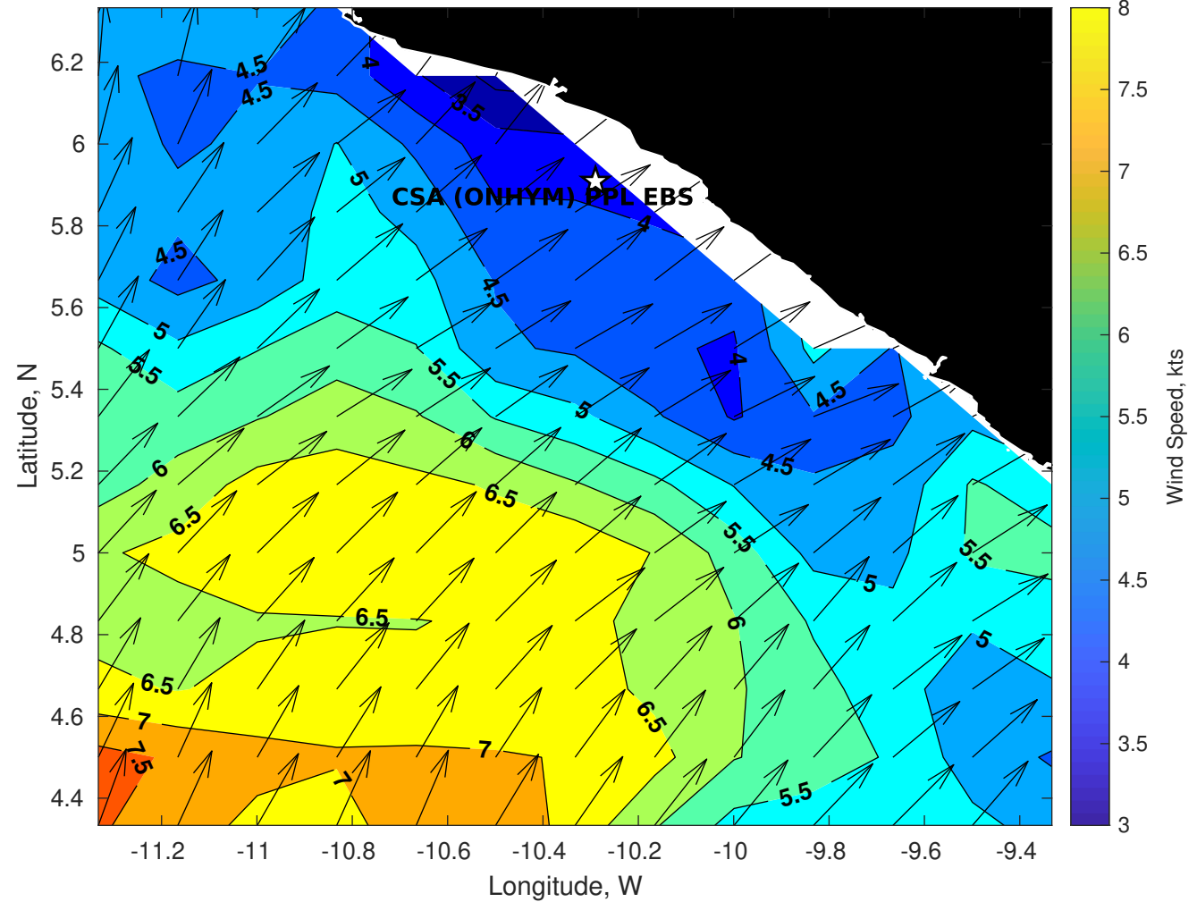
GFS Winds (kts) for CSA (ONHYM) PPL EBS - Liberia at 24-Dec-2025 09:00:00
