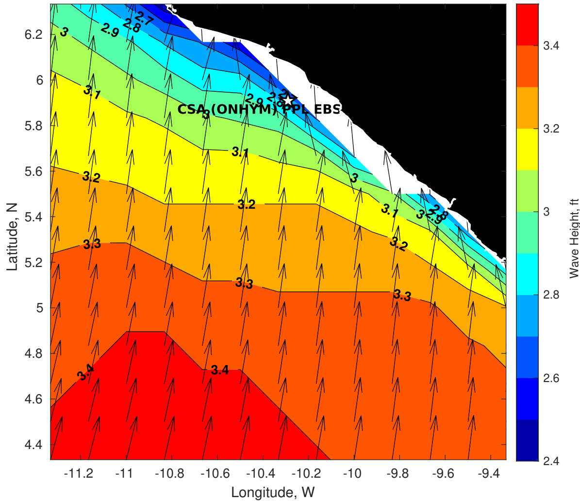
GFS Wave Height (ft) for CSA (ONHYM) PPL EBS - Liberia at 24-Dec-2025 09:00:00
