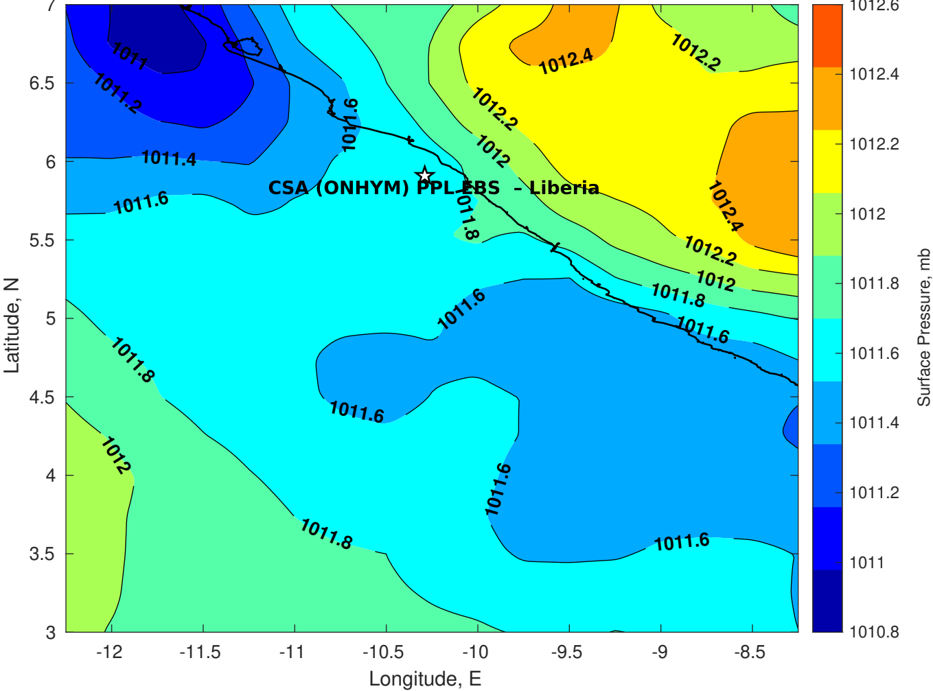
Surface Pressure (mb) for CSA (ONHYM) PPL EBS - Liberia at 26-Dec-2025 00:00:00
