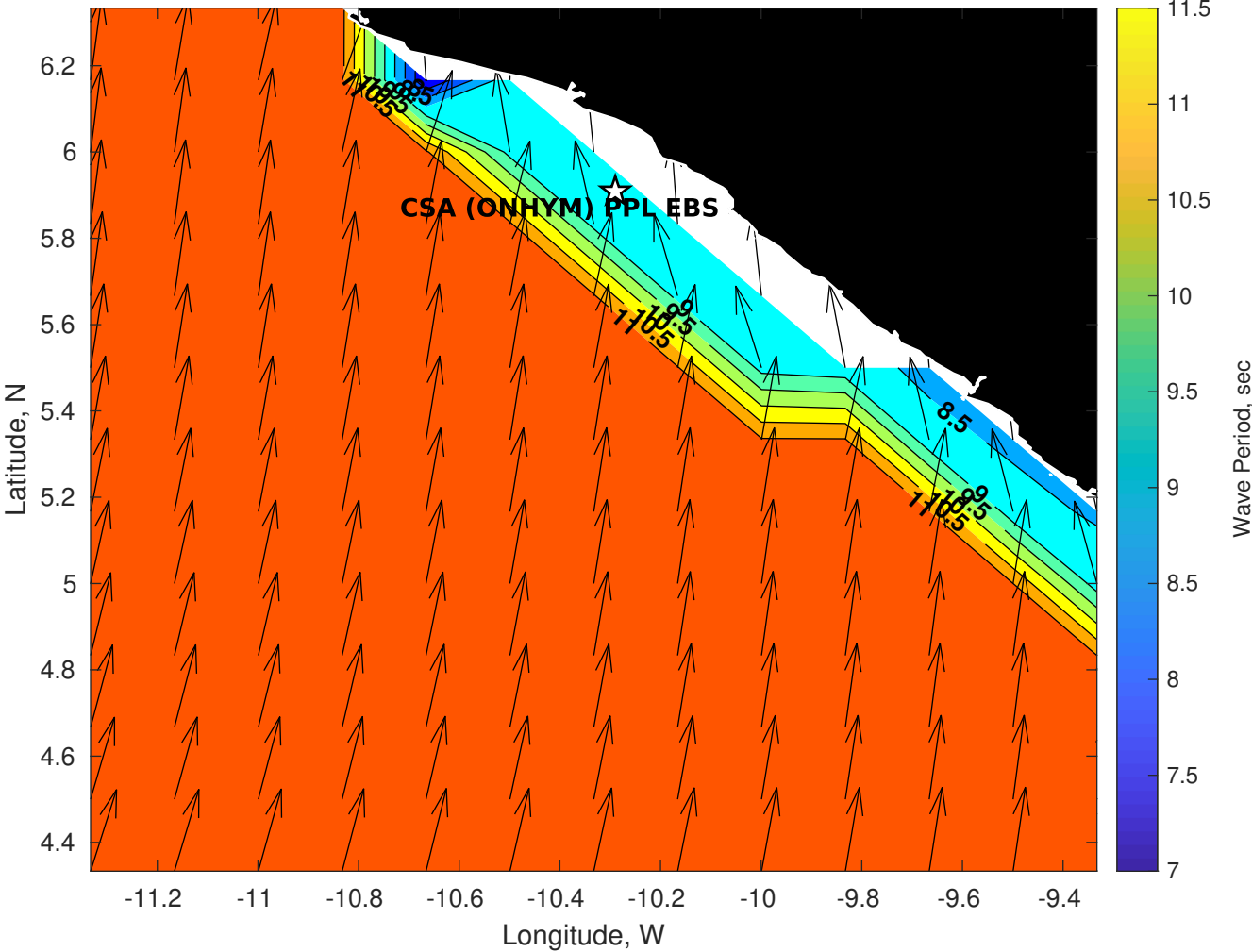
GFS Wave Period (sec) for CSA (ONHYM) PPL EBS - Liberia at 24-Dec-2025 09:00:00
