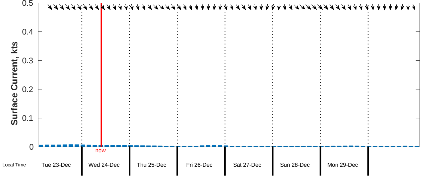
Surface Current Forecast for CSA (ONHYM) PPL EBS - Liberia from 23-Dec-2025 00:00:00 to 31-Dec-2025 00:00:00
