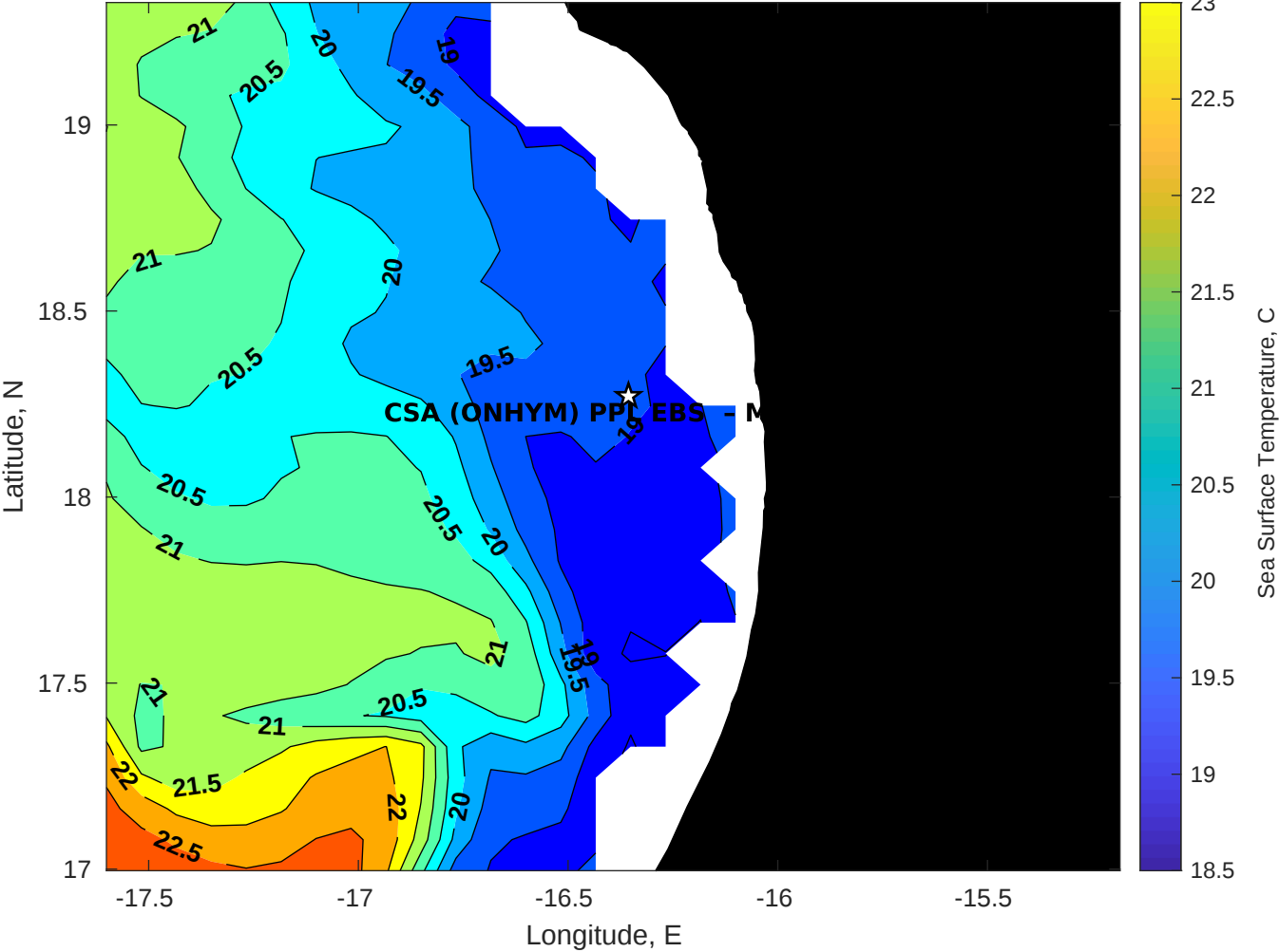
SST for CSA (ONHYM) PPL EBS - Mauritania at 23-Dec-2025 00:00:00
