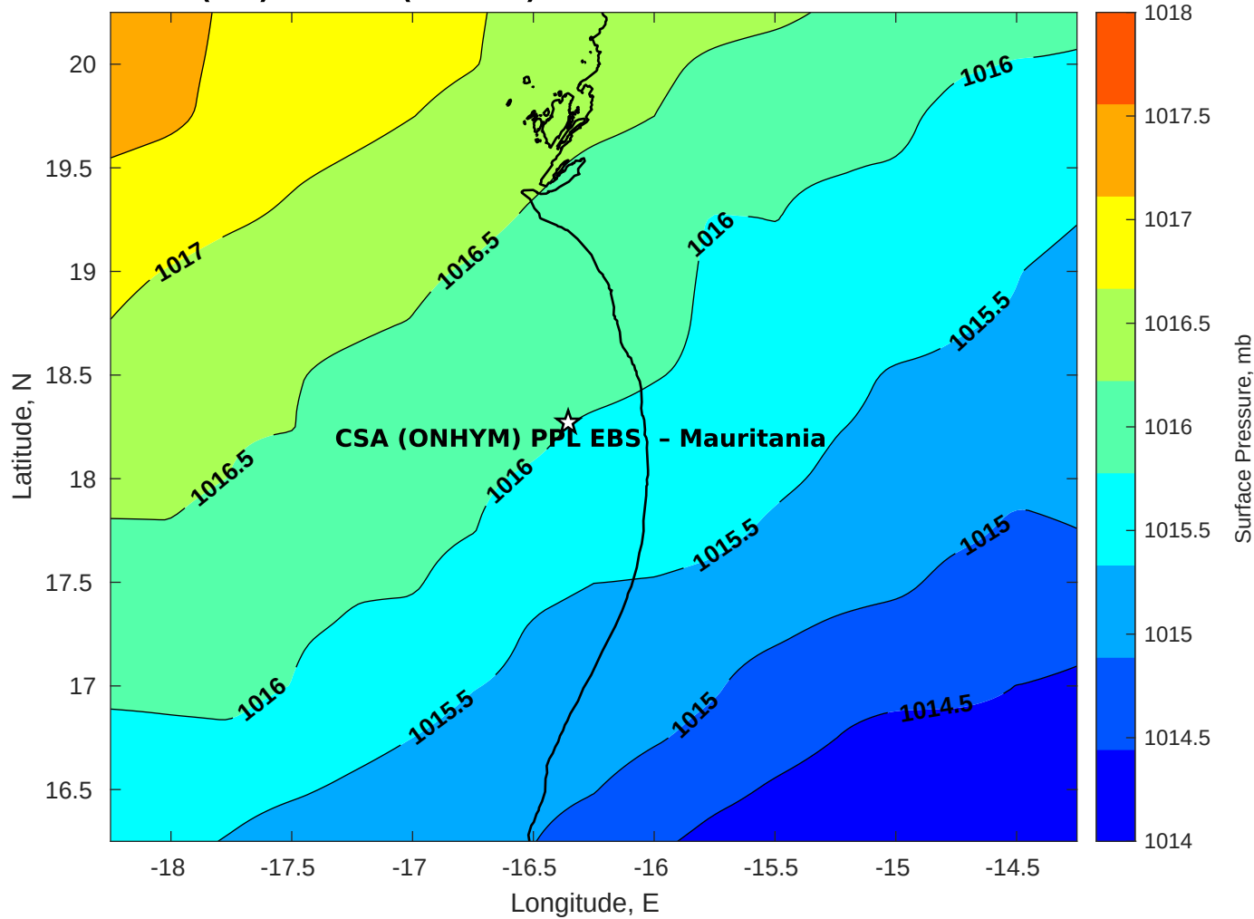
Surface Pressure (mb) for CSA (ONHYM) PPL EBS - Mauritania at 26-Dec-2025 00:00:00
