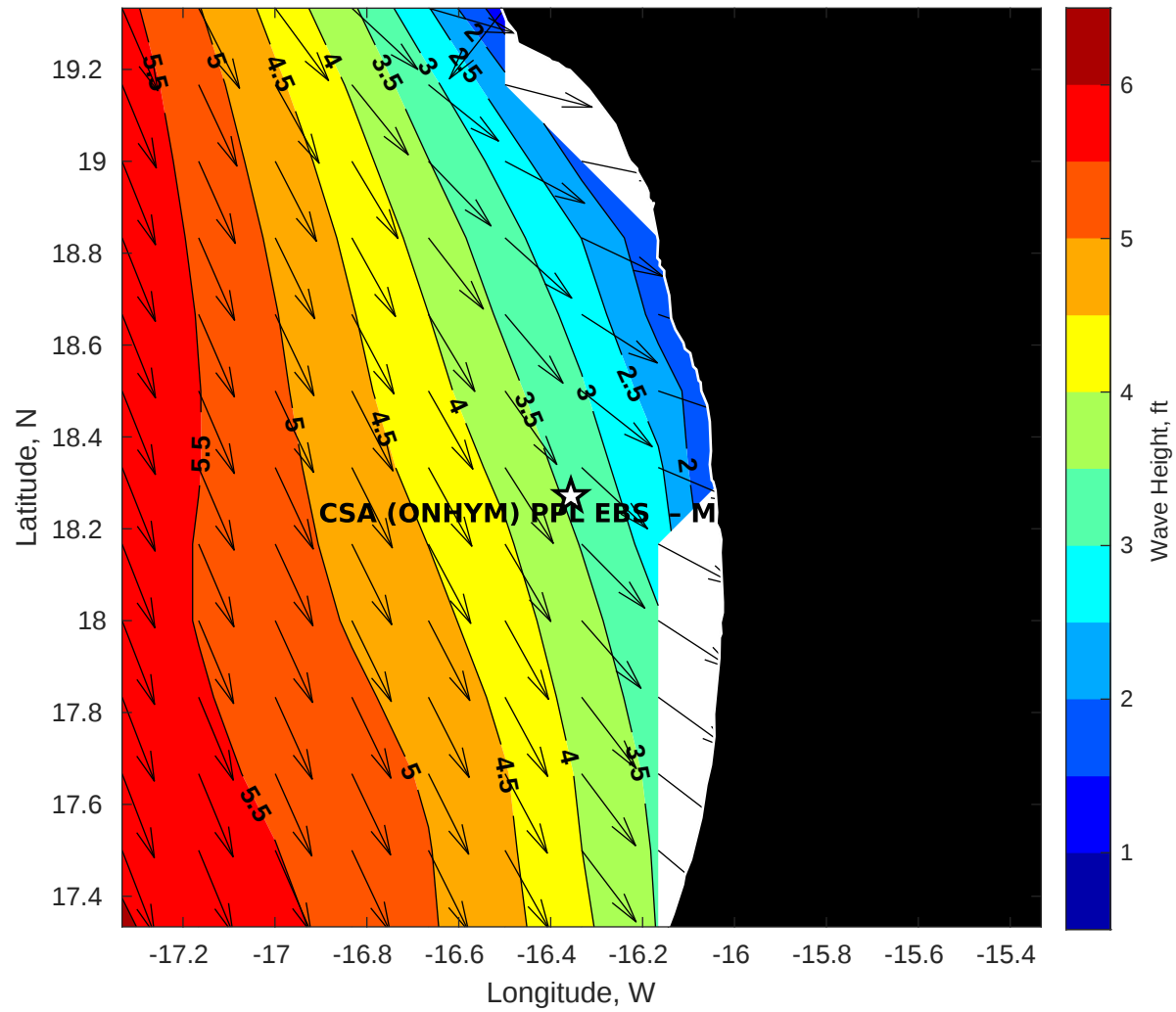
GFS Wave Height (ft) for CSA (ONHYM) PPL EBS - Mauritania at 24-Dec-2025 09:00:00
