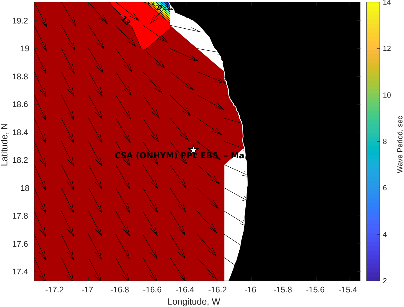
GFS Wave Period (sec) for CSA (ONHYM) PPL EBS - Mauritania at 24-Dec-2025 09:00:00
